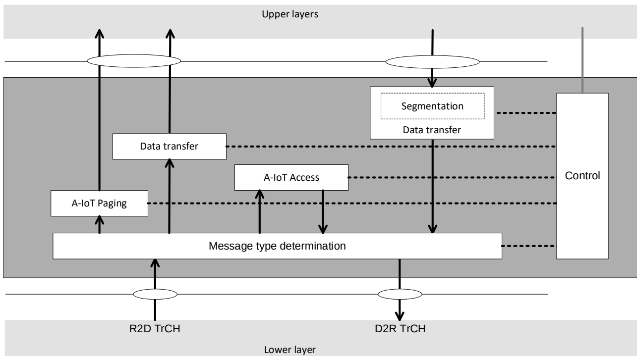
Figure 4.2-1: A-IoT MAC structure overview
