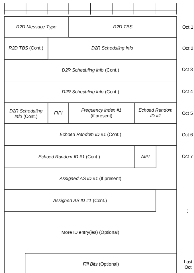
Figure 6.2.1.3-1: MAC PDU of Random ID Response message
