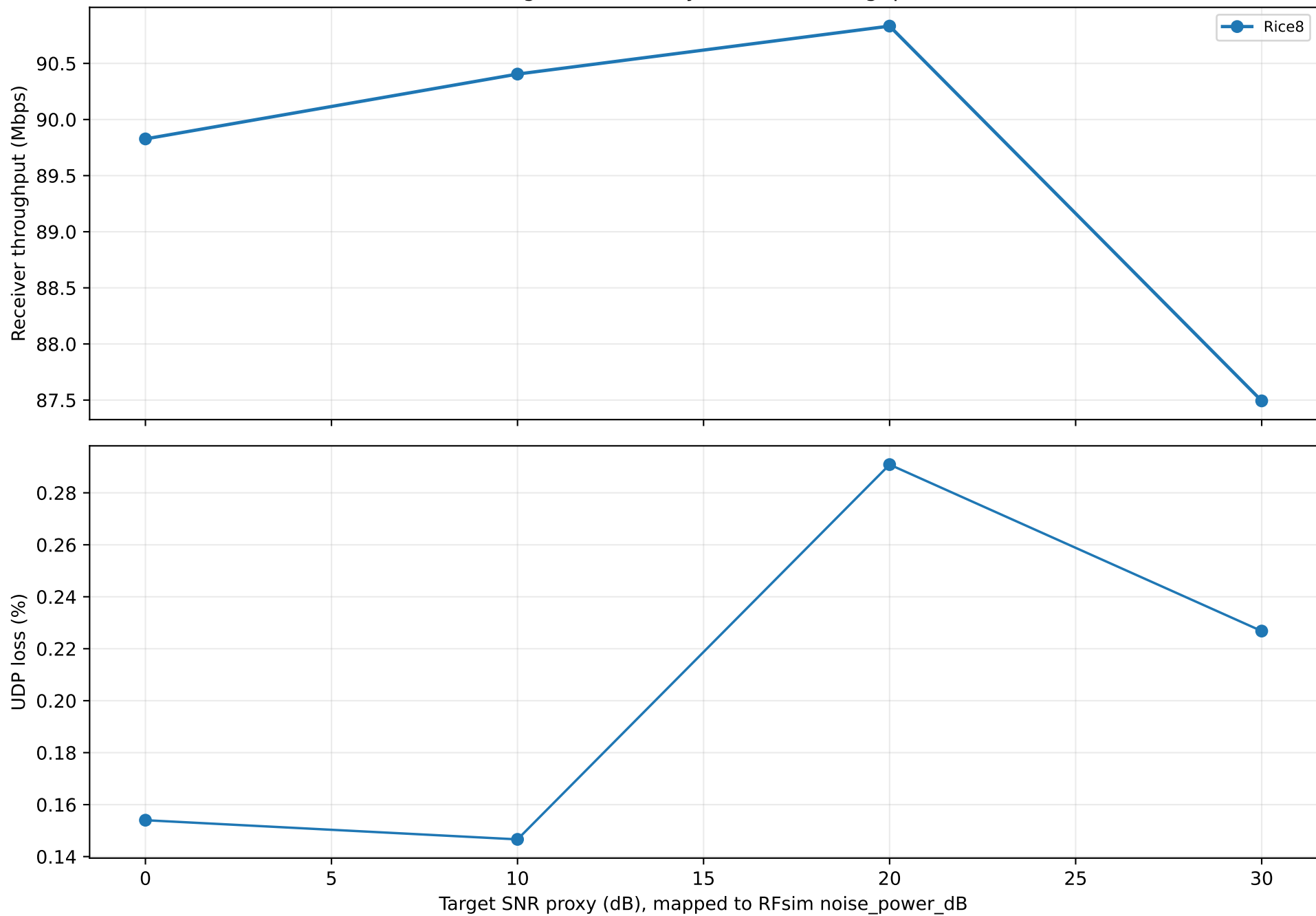
PAPER-08 Fig.9 RFsim Proxy: UDP DL Throughput vs SNR
