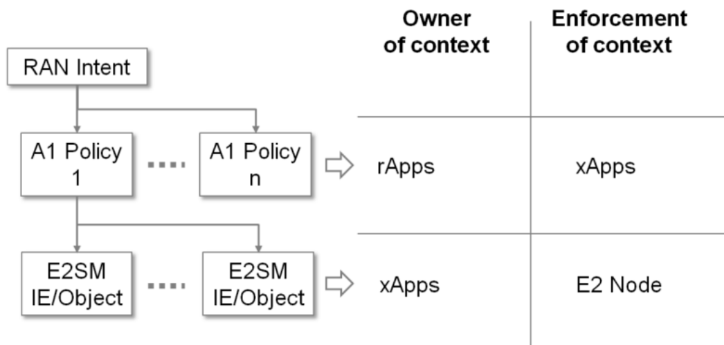
Figure 4.1- 1: Context for each layer
