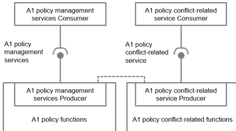
Figure B.1-2: Diagram for the potential realization of option.2 (A1 policy conflict-related service separate from A1 policy management services)
