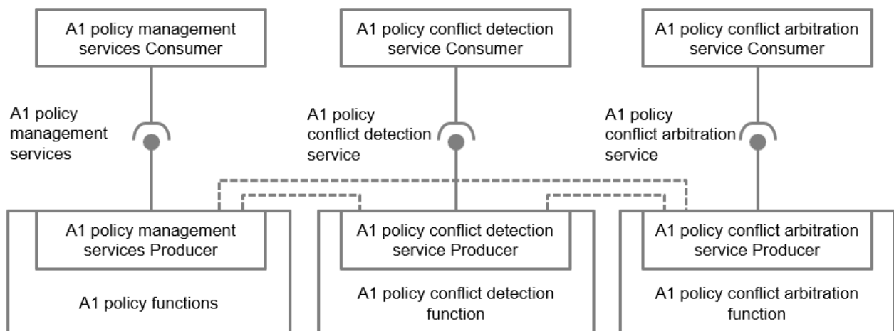
Figure B.1-3: Diagram for the potential realization of option.3 (Individual A1 policy conflict detection and A1 policy conflict arbitration services)
