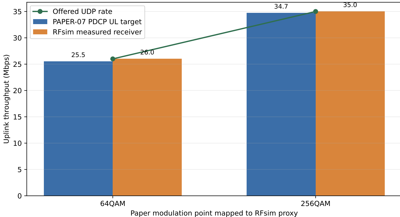
PAPER-07 Uplink Peak Rate Reproduction Proxy
