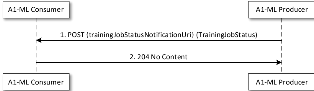
Figure 5.4.3.5.1-1: Notify AI/ML model training job status operation
