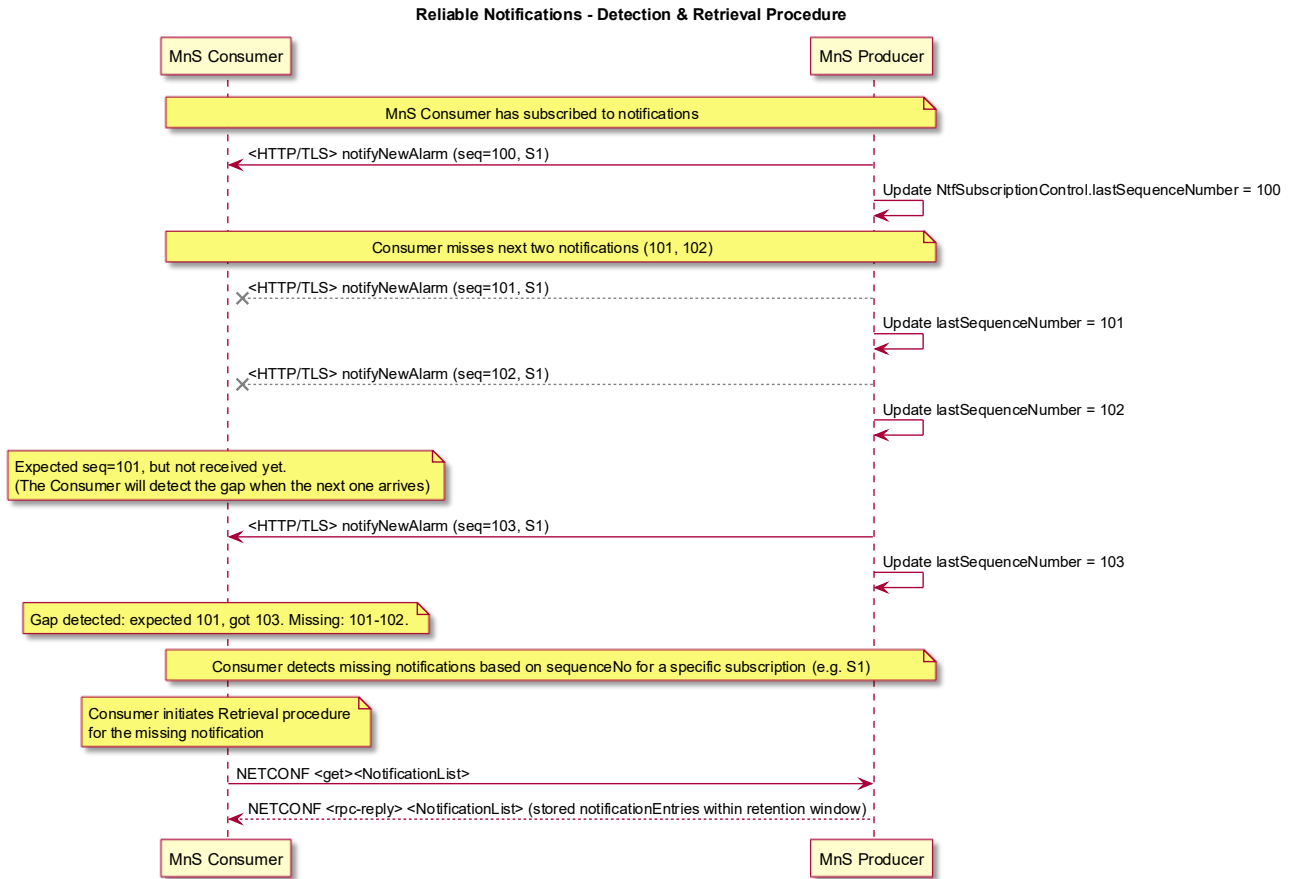
Figure E-1: Reliable notifications Detection & Retrieval Procedure example
