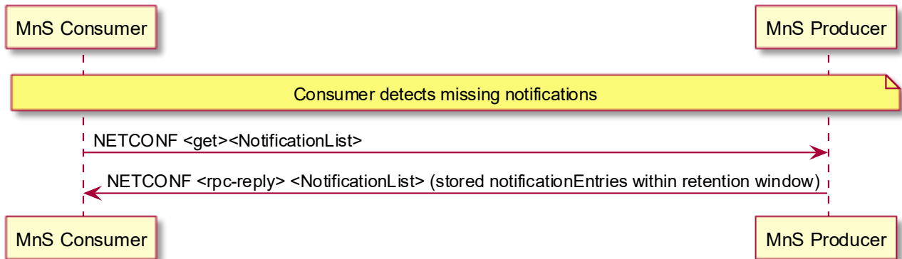
Figure 6.11.3.3.3-2 Retrieve Procedure for Reliable Notifications
