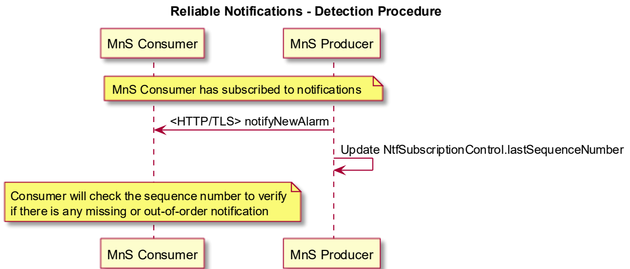
Figure 6.11.3.3.2-1 Detection Procedure for Reliable Notifications
