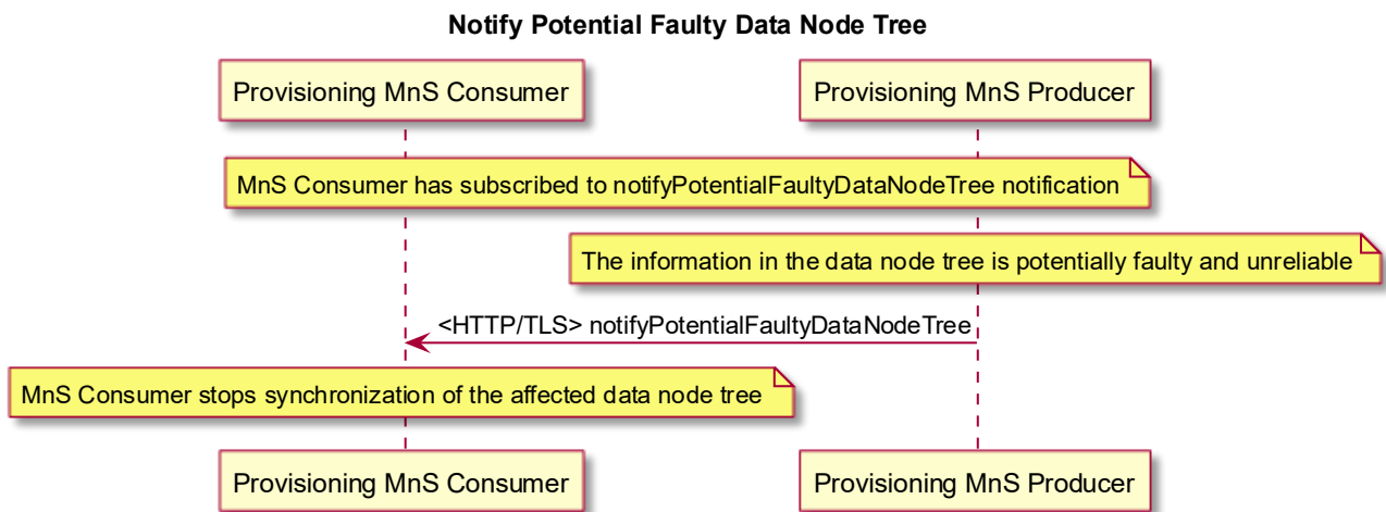
Figure 6.1.14.2-1 Notify Potential Faulty Data Node Tree
