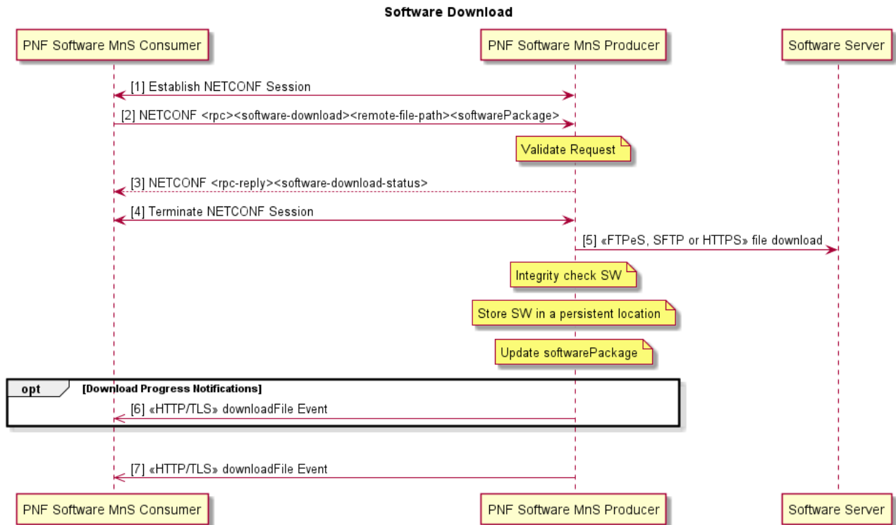
Figure 6.8.3.3-1 Software Download
