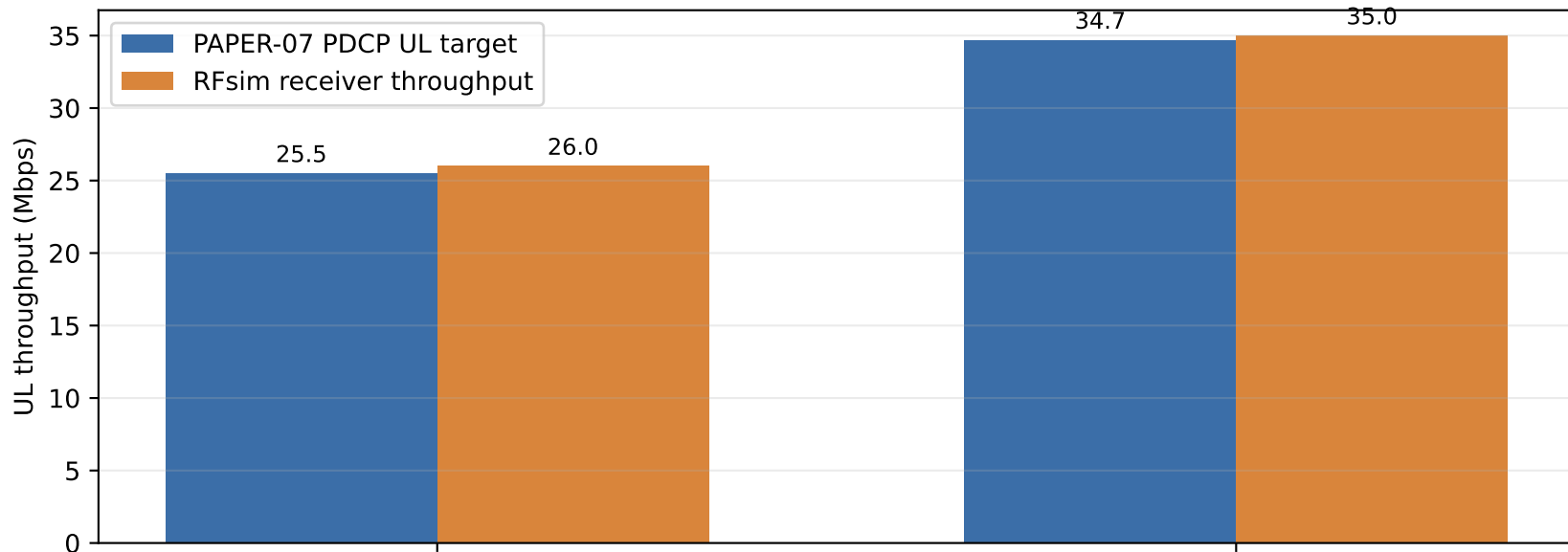
PAPER-07 True 256QAM UL Retest
