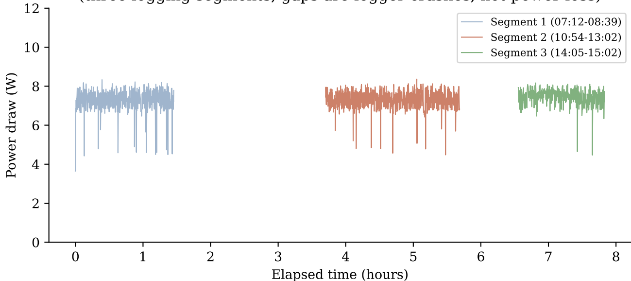
Measured power draw across the battery drain (three logging segments; gaps are logger crashes, not power loss)
