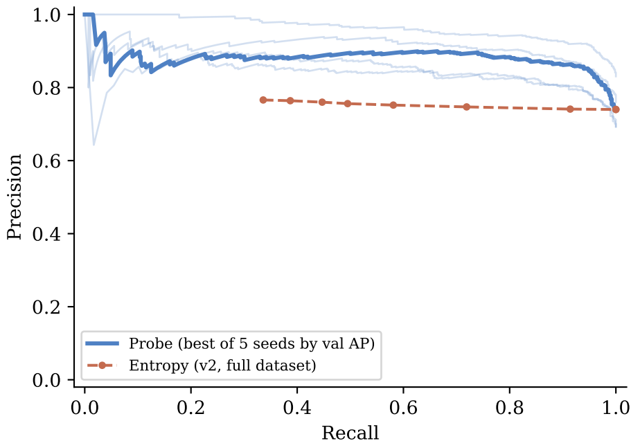
Probe vs. entropy, v2 data (test AP: 0.890 \pm 0.045 across 5 seeds)
