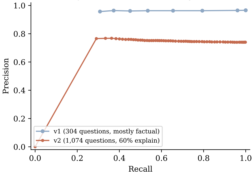
Entropy baseline: small vs. large dataset
