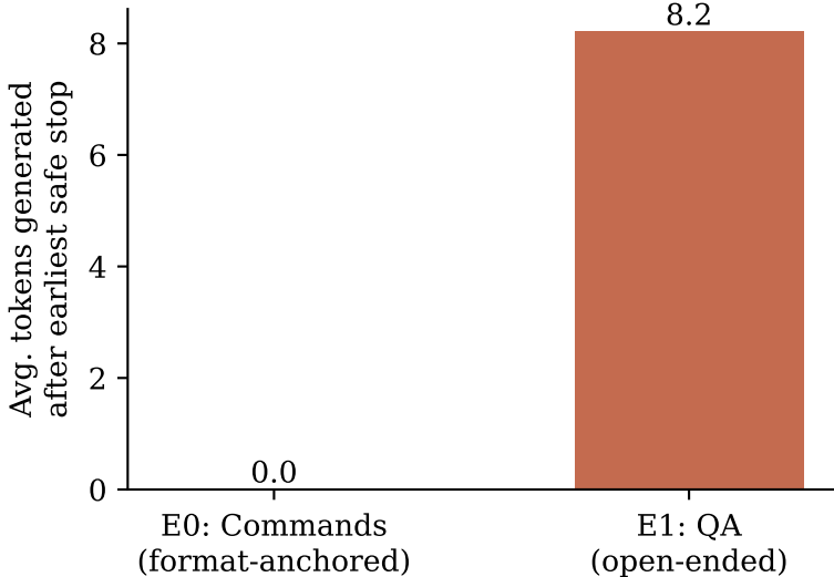
Post-answer waste by task type
