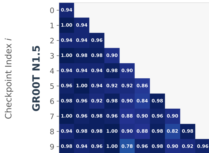
LIBERO-Spatial
