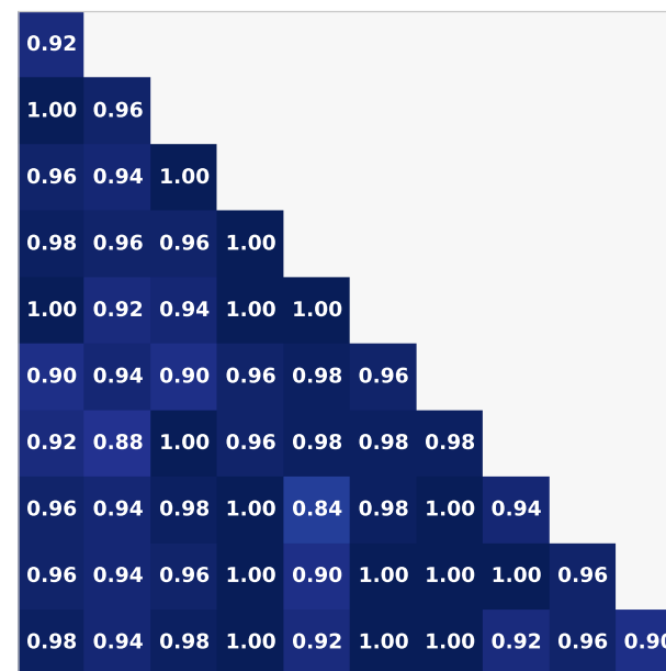
LIBERO-Object
