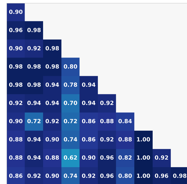
LIBERO-Goal
