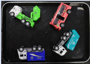
(b) Seen
