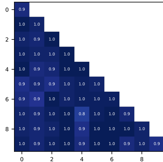
GR00T N1.5
