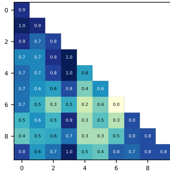
BC-Transformer
