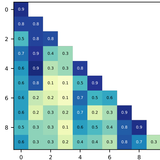
BC-Transformer
