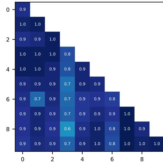
GR00T N1.5
