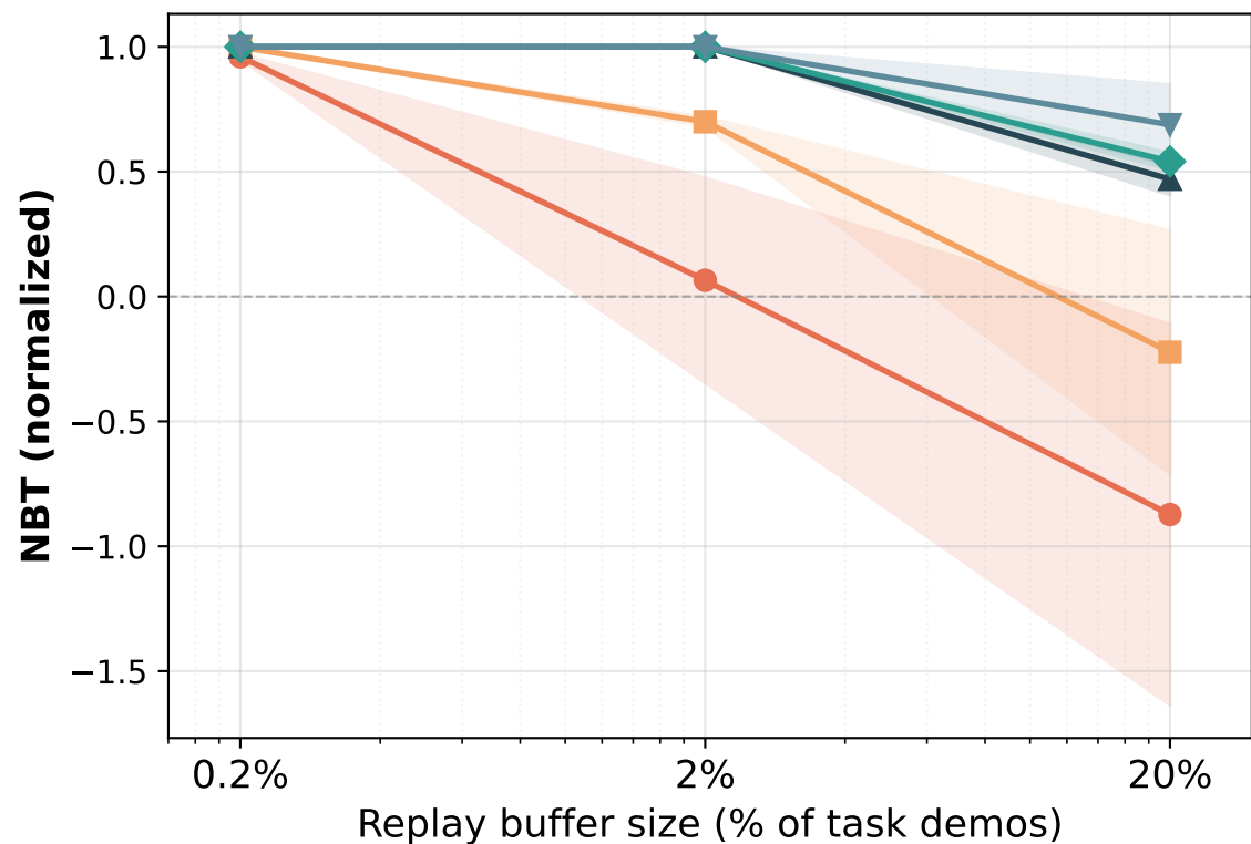
LIBERO-10: Normalized NBT
