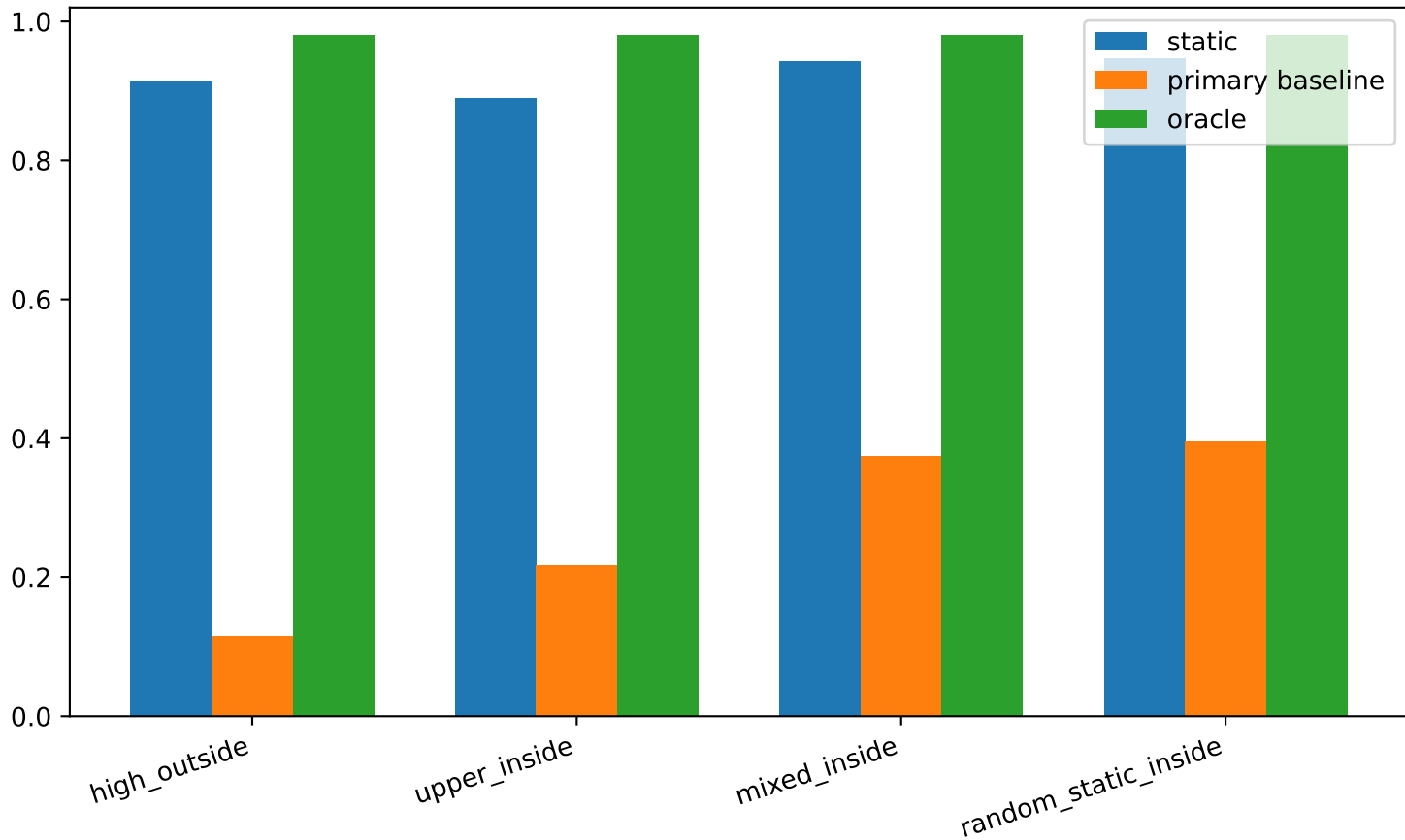
Crossing probability by T=200
