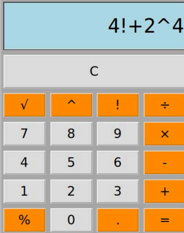
Factorial and power function
