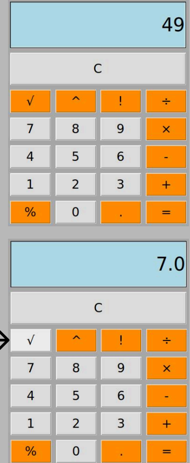
Square root function
