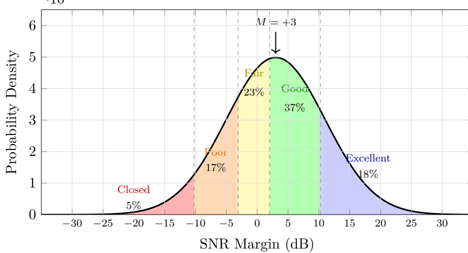
Tier Probability Distribution ( M = +3 dB, \sigma = 8 dB, ionocast 0.90/0.60/0.35/0.10 boundaries)
