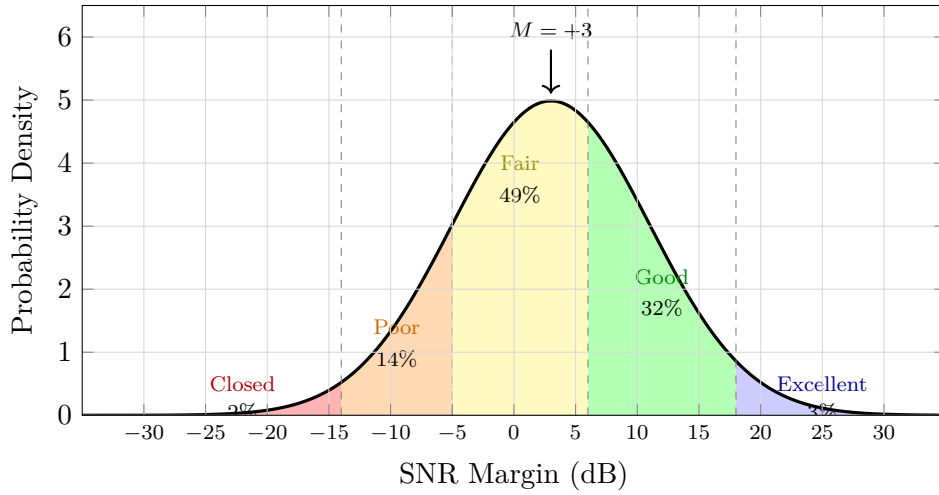
Tier Probability Distribution ( M = +3 dB, \sigma = 8 dB, fixed-dB boundaries +18 / +6 / -5 / -14 )
