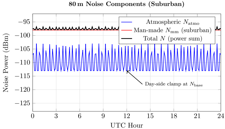
Figure 5: Noise power components on 80 m in a suburban environment (post-2026-04-30 re-anchor: N_{\text{base}} = -113 dBm). The man-made noise ( -98 dBm) dominates at all hours; the atmospheric night-side swing barely affects the total, and the day side is clamped at the galactic base. Power-summing the two components in linear units (the model used here) gives the black curve, which sits essentially at the man-made level since 10^{-113/10} + 10^{-98/10} \approx 10^{-98/10} when the components differ by \sim 15 dB. An earlier formulation that combined the two by an incorrect dB-domain operation produced a noise estimate several dB above the man-made-dominated truth on suburban / urban sites, inflating the margin and biasing verdicts open; the power-sum form is therefore a correctness constraint, not a stylistic choice.
