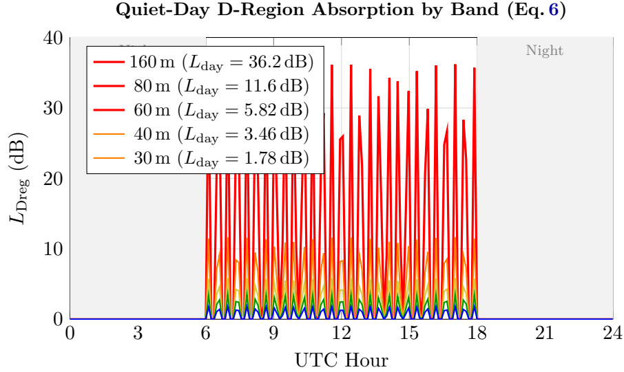
Figure 6: Quiet-day D-region absorption by band under the L_{\text{day}}(f) \cdot \cos^{0.7}(\chi) form of Eq. 6. 160 m reaches 36.2 dB at local noon (at the 1.85 MHz reference plotted; the 1.838 MHz band anchor gives 36.6); 30 m and above are essentially unaffected. Night absorption is zero. The illustrative curves show a smooth descent toward zero at low \cos \chi , but the actual implementation hard-gates L_{\text{Dreg}} = 0 at \cos \chi < 0.05 (Eq. 6); the figure smooths that gate for readability rather than showing the cliff. The grayline bonus of §5.5 adds a terminator-peaked Gaussian credit (peak \min(15 \text{ dB}, L_{\text{day}}) ) alongside the day-side charge plotted here.
