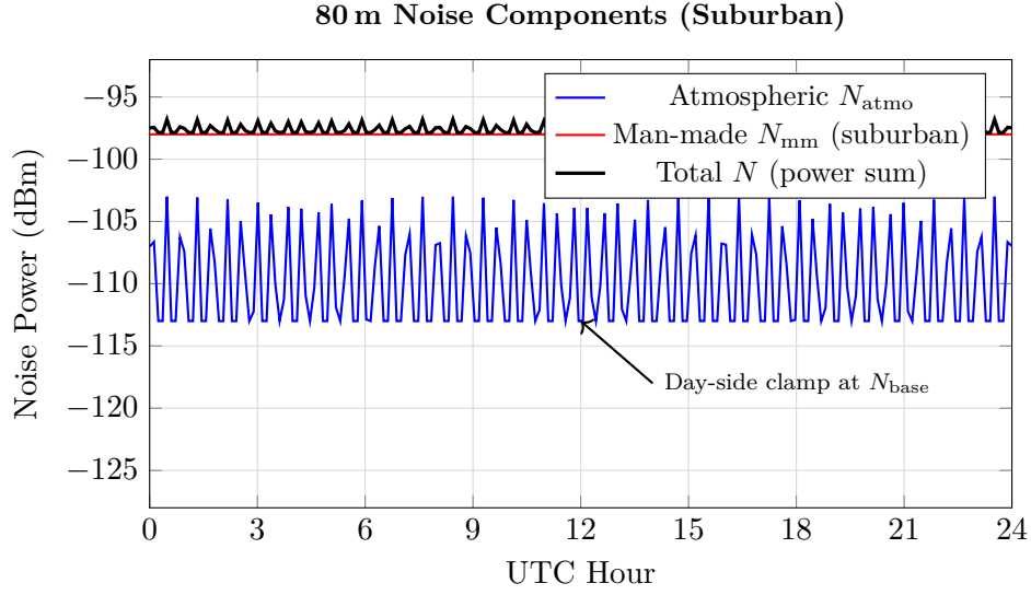
Figure 5: Noise power components on 80 m in a suburban environment (post-2026-04-30 re-anchor: N_{\text{base}} = -113 dBm). The man-made noise (-98 dBm) dominates at all hours; the atmospheric night-side swing barely affects the total, and the day side is clamped at the galactic base. Power-summing the two components in linear units (the model used here) gives the black curve, which sits essentially at the man-made level since 10^{-113/10} + 10^{-98/10} \approx 10^{-98/10} when the components differ by \sim 15 dB. An earlier formulation that combined the two by an incorrect dB-domain operation produced a noise estimate several dB above the man-made-dominated truth on suburban / urban sites, inflating the margin and biasing verdicts open; the power-sum form is therefore a correctness constraint, not a stylistic choice.
