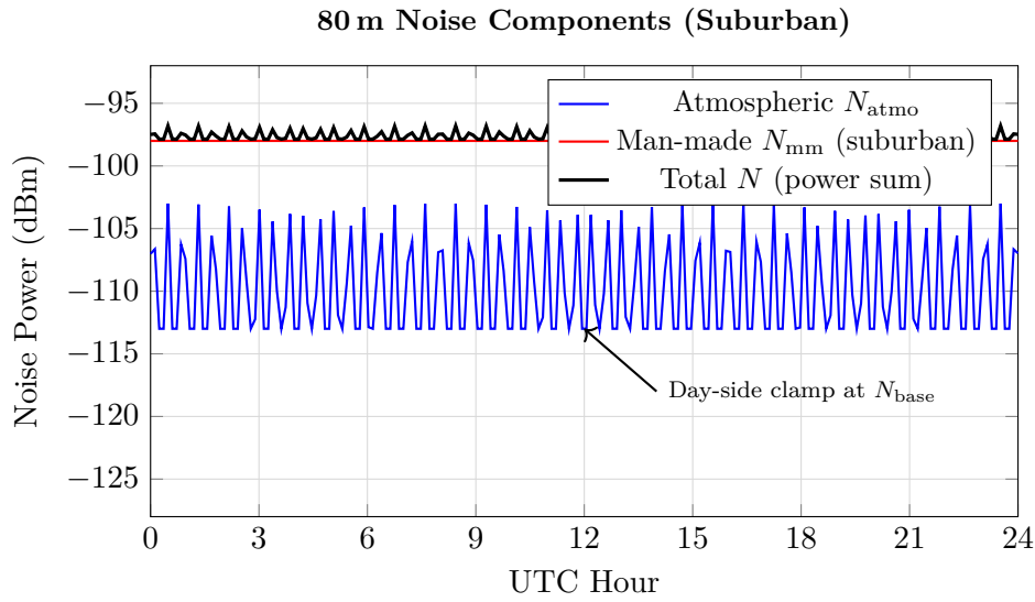
Figure 5: Noise power components on 80 m in a suburban environment ( N_{\text{base}} = -113 dBm). The man-made noise ( -98 dBm) dominates at all hours; the atmospheric night-side swing barely affects the total, and the day side is clamped at the galactic base. Power-summing the two components in linear units (the model used here) gives the black curve, which sits essentially at the man-made level since 10^{-113/10} + 10^{-98/10} \approx 10^{-98/10} when the components differ by \sim 15 dB. Combining the two by a dB-domain operation instead would produce a noise estimate several dB above the man-made-dominated truth on suburban / urban sites, inflating the margin and biasing verdicts open; the power-sum form is therefore a correctness constraint, not a stylistic choice.
