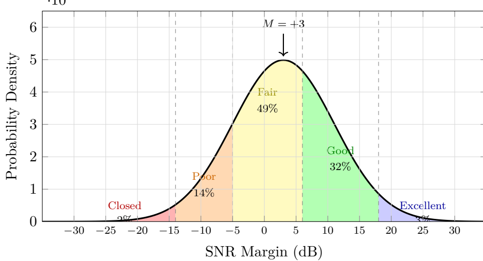
Tier Probability Distribution ( M = +3 dB, \sigma = 8 dB, fixed-dB boundaries +18 / +6 / -5 / -14)
