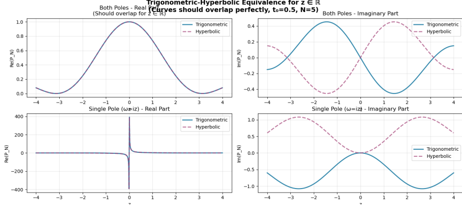
Figure 1.4: Equivalence between \Re(\mathbb{P}_N[\text{sinc} * \delta(t - t_0)](z)) for different contours
