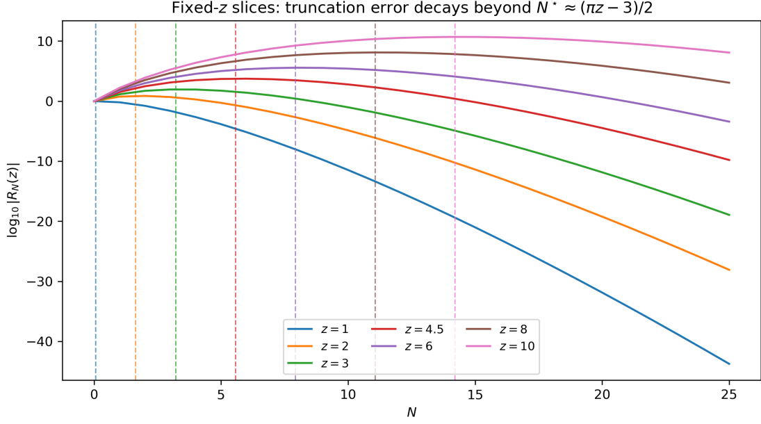
Figure 1.2: Logarithmic plot of the remainder term where the common definition given for \text{sinc}, \text{sinc}(\pi z) , is used. The decay point N^* \approx \frac{\pi z - 3}{2} \propto z reflects the ( trivial ) fact that higher z needs a compensatory higher N for lower absolute error |\mathbb{E}| . Note: Per(??) \forall z \in a, |\mathbb{E}_N(z)| \gg \forall z \in b even though |R_N(a)| < |R_N(b)| can hold true for a \in [0, N^*), b \in [N^*, \infty)
