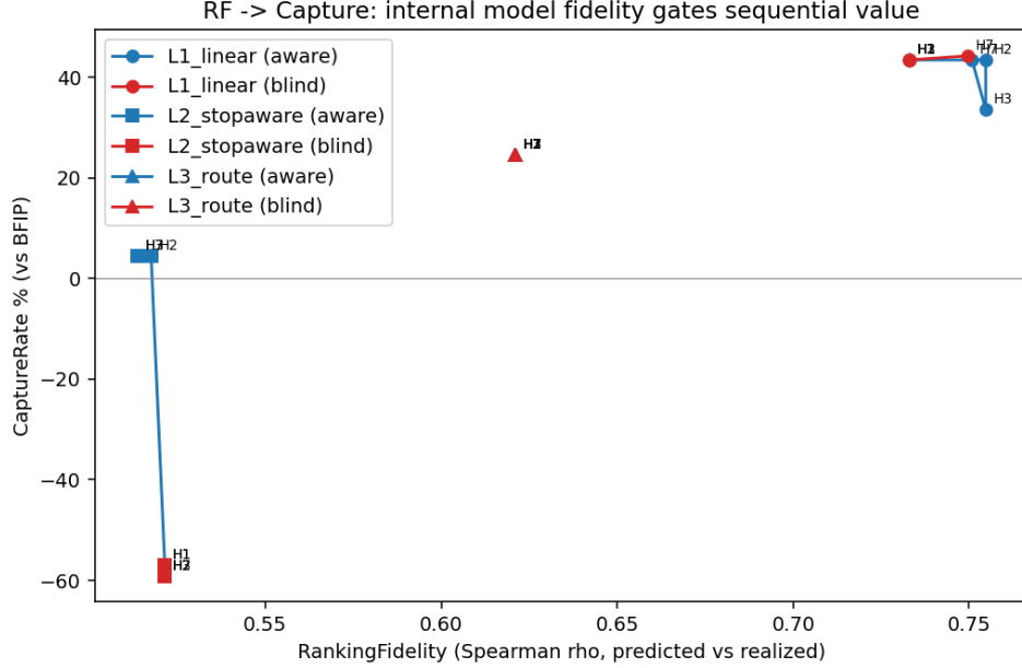
Figure 3: Ranking Fidelity vs. Capture Rate: each point is a (model, horizon) configuration; x-axis = Spearman \rho between predicted and realized per-expert cost rankings; y-axis = Oracle Opportunity Capture Rate. Capture does not increase monotonically with \rho : the crudest model (L1) achieves the highest capture via implicit conservatism.
