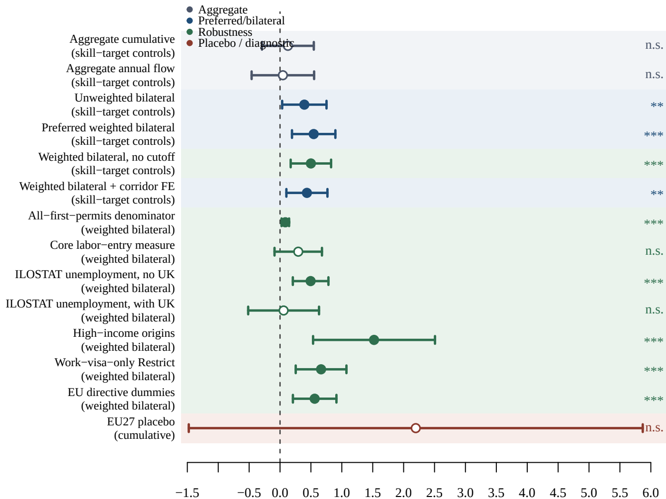
Graph 2. Coefficients across main, robustness, and placebo specifications
