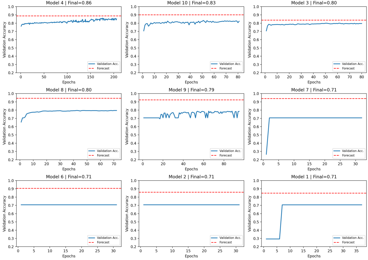
Figure 6.3: Example of learning curves for several models with their respective forecasted accuracy on the phoneme dataset.
