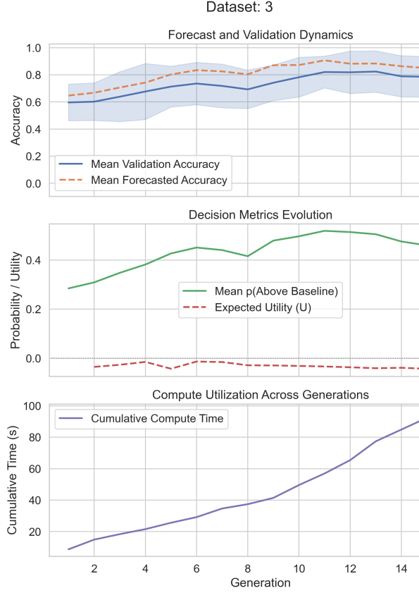
Figure 6.5: Generation-level dynamics for Dataset 3. The figure summarizes how validation accuracy, forecasted performance, probability of surpassing the baseline, and expected utility evolved through successive generations of the ShouldYouEvenNN framework.
