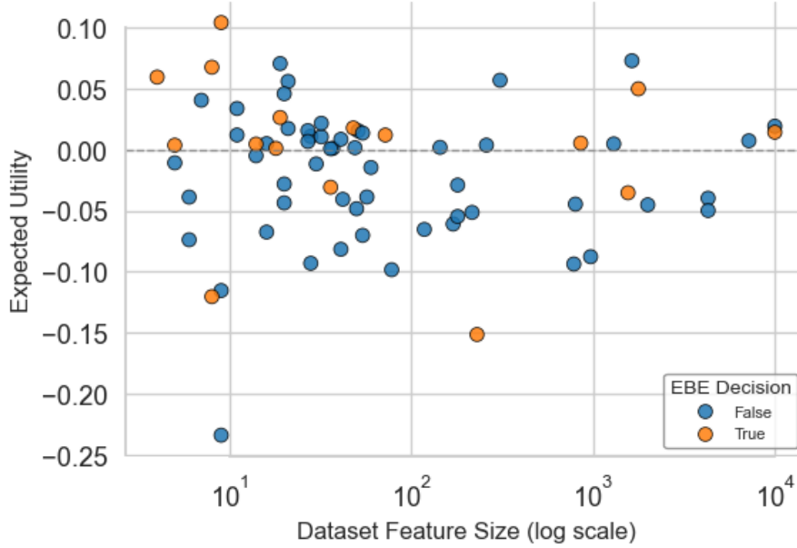
Figure 6.6: Dataset Feature Size vs U
