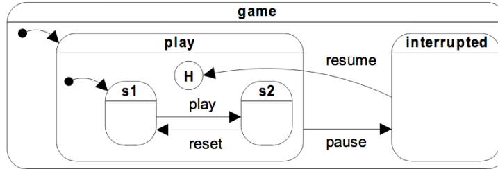
Fig. 6.2 Pause-and-resume via hierarchy and history state in the game controller.
