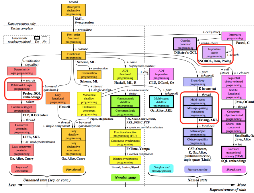
Fig. 2.2 A taxonomy of programming paradigms due to Peter Van Roy.
