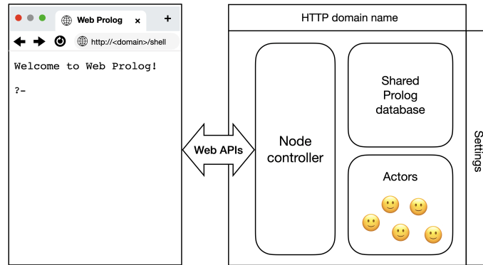
Fig. 3.4 The anatomy of a Prolog node. A terminal running in a web browser is attached to it.
