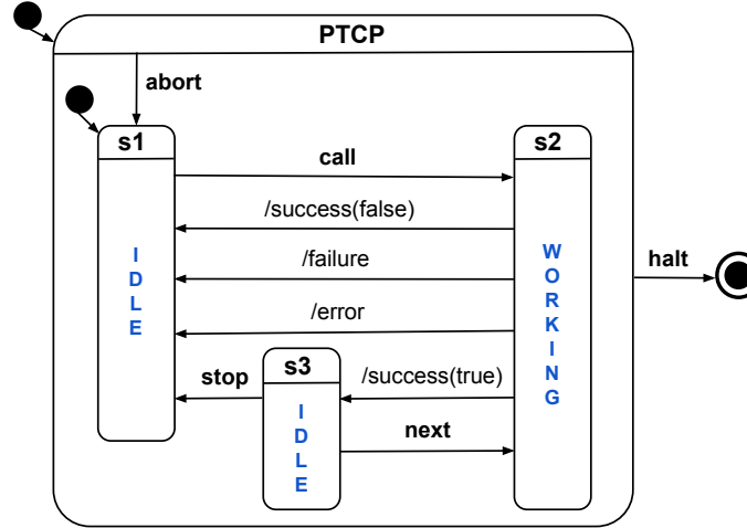
Fig. 3.3 Statechart specifying the Prolog Toplevel Communication Protocol (PTCP). Bold transitions denote messages sent from the client to the toplevel, whereas transitions prefixed by '/' denote responses sent by the toplevel back to the client.
