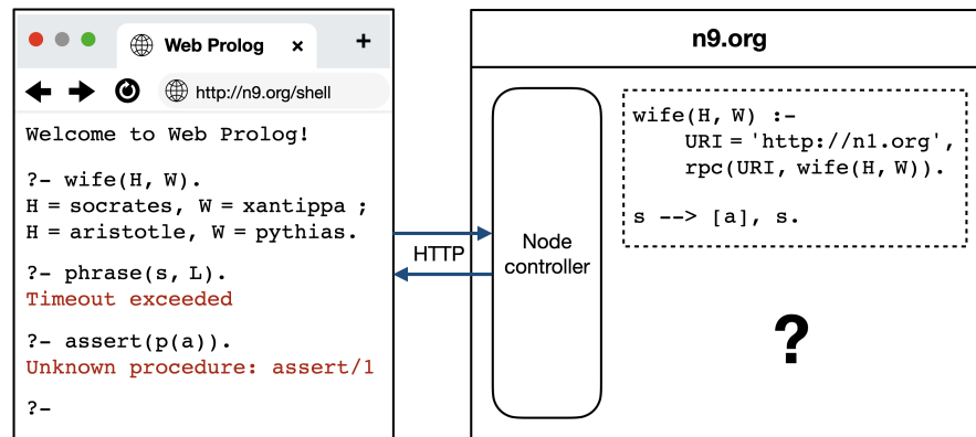
Fig. 3.10 Stateless interaction between a web browser and an ISOBASE node.
