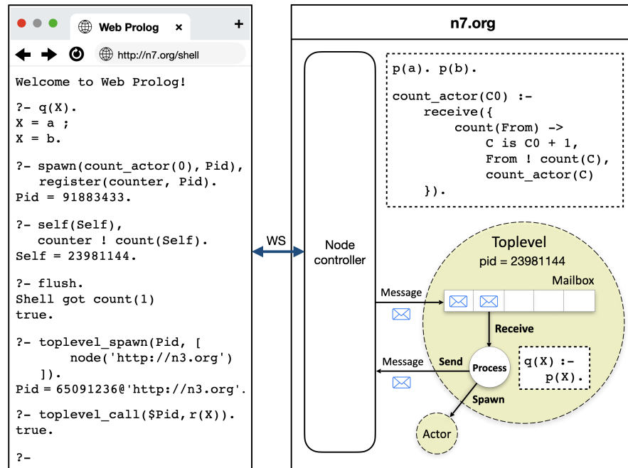
Fig. 3.18 A scenario involving a web browser in conversation with a remote node running a toplevel actor over a stateful WebSocket connection.
