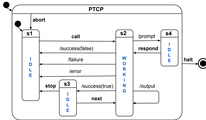
Fig. 3.20 Statechart specifying the PTCP for a successful conversation with a toplevel over HTTP.
