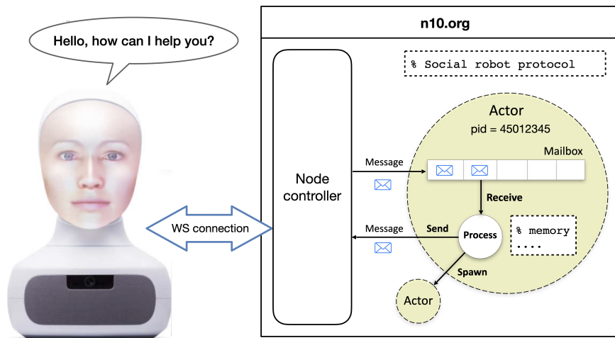
Fig. 3.13 Stateful interaction between a social robot and a remote ACTOR node.
