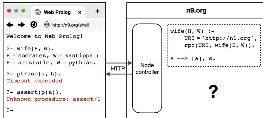
Fig. 3.16 Stateless interaction in a scenario involving a web browser and a remote node.
