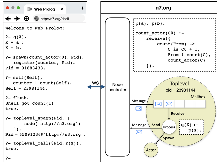
Fig. 3.12 A browser in conversation with a remote ACTOR node running a toplevel actor over a stateful WebSocket connection.
