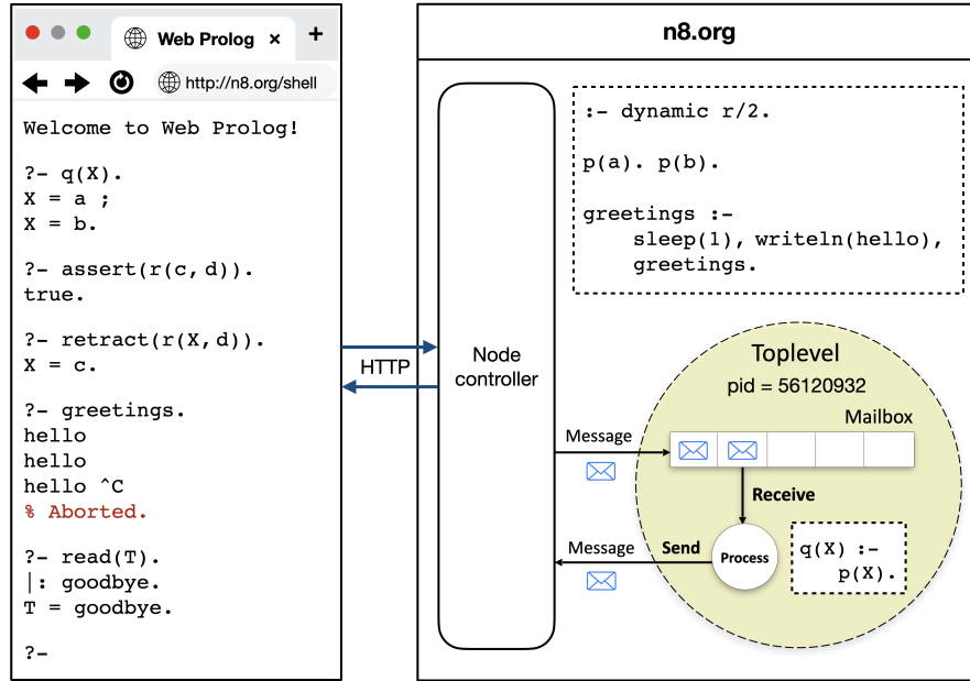
Fig. 3.11 A browser in conversation over semi-stateful HTTP with a remote ISOTOPE node running a toplevel actor.
