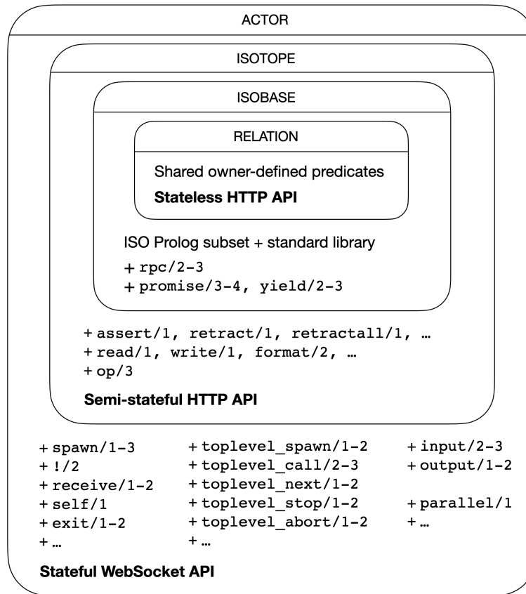
Fig. 3.14 The profile hierarchy. Each ring adds requirements to those of the profiles inside it.
