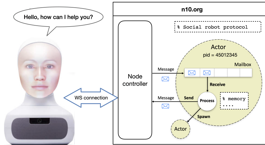
Fig. 3.19 Stateful interaction in a scenario involving a social robot and a remote ACTOR node.
