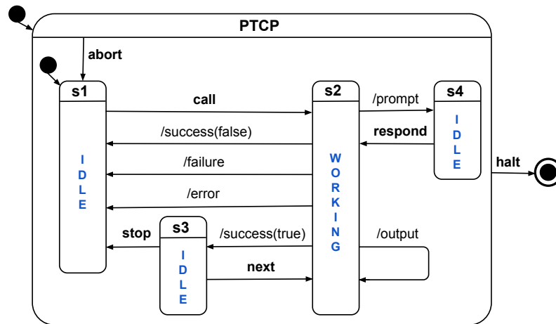
Fig. E.1 Statechart specifying the PTCP for a successful conversation with a toplevel over HTTP.
