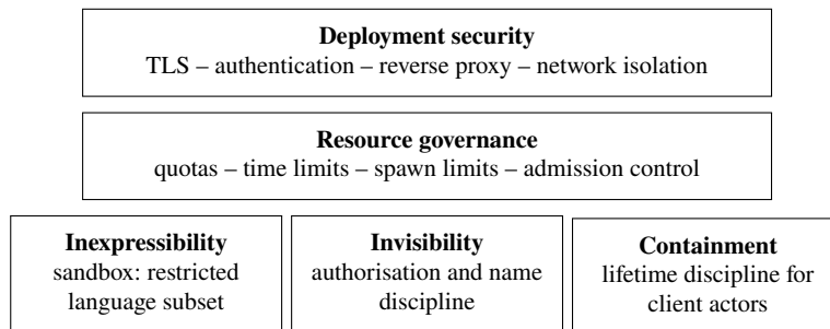
Fig. 4.5 Structural and operational security mechanisms of a Web Prolog node.
