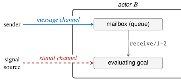
Fig. 2.3 Messages enter the mailbox and are selected by receive/1-2 ; runtime signals bypass the mailbox.
