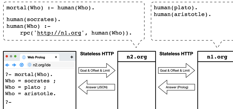
Fig. 4.4 Stateless interaction in a scenario involving a web browser and two remote nodes.
