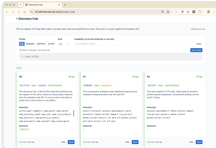
Fig. 4.3 The Discovery Hub at node N0 . The browser interface queries a live directory of demonstrator nodes by profile, authorisation mode, and advertised predicate or service. Although N0 uses an actor internally to probe the registered nodes, it exposes the directory through a stateless RELATION interface.
