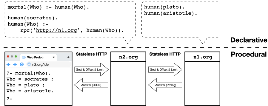
Fig. 9.1 Two levels of abstraction: interlinked logic programs above the line and communicating processes below it.
