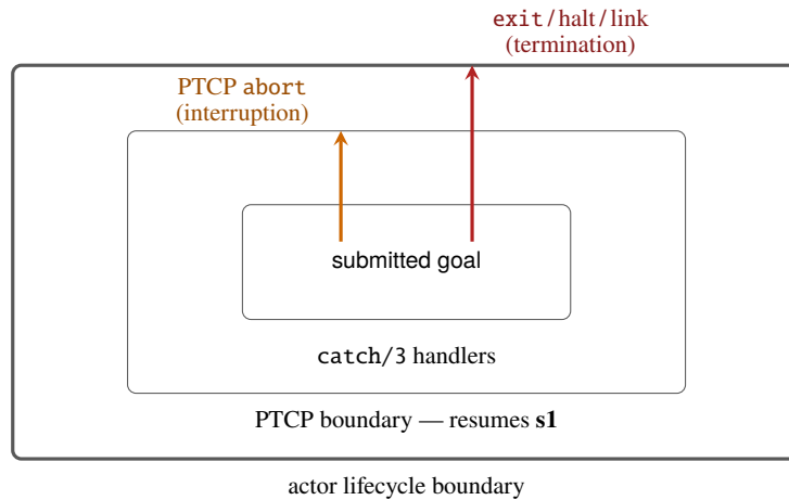
Fig. 3.4 Abort crosses client exception handlers but stops at the PTCP boundary; termination crosses the actor lifecycle boundary. Cleanup runs during either unwind.
