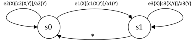
Fig. 2.5 A simple event-driven state machine. s0 is the initial state.
