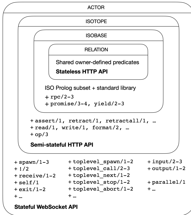
Fig. 3.8 The node-profile hierarchy. Each profile includes the requirements of those inside it.
