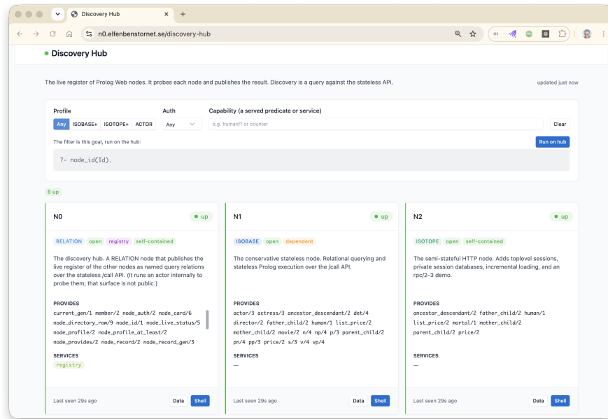
Fig. 4.2 The Discovery Hub at node N0. The browser interface queries a live directory of demonstrator nodes by profile, authorisation mode, and advertised predicate or service. Although N0 uses an actor internally to probe the registered nodes, it exposes the directory through a stateless RELATION interface.
