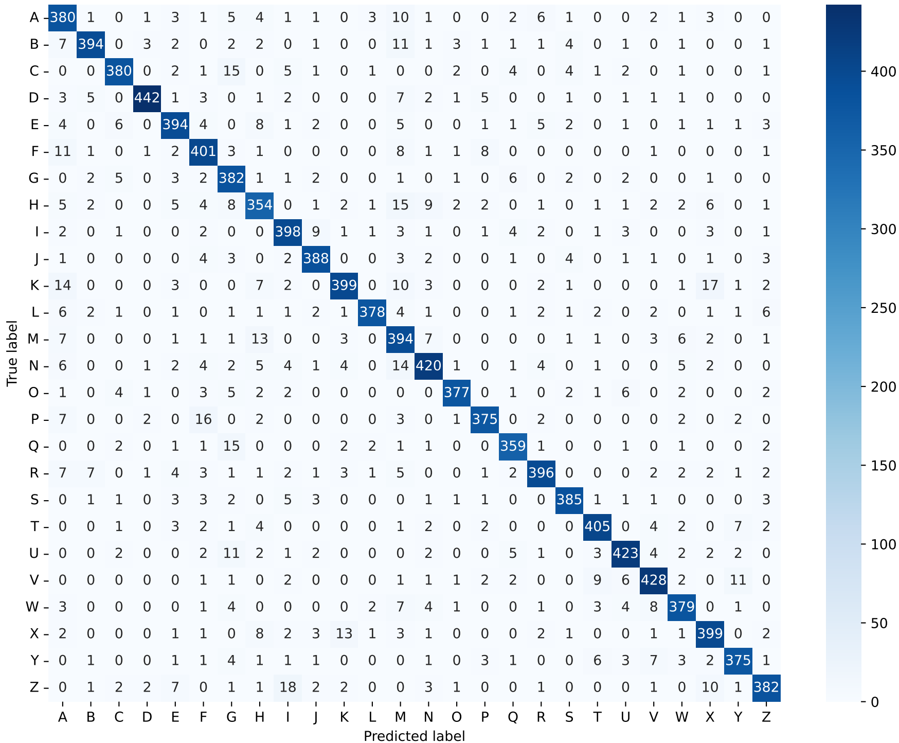
Test Confusion Matrix
