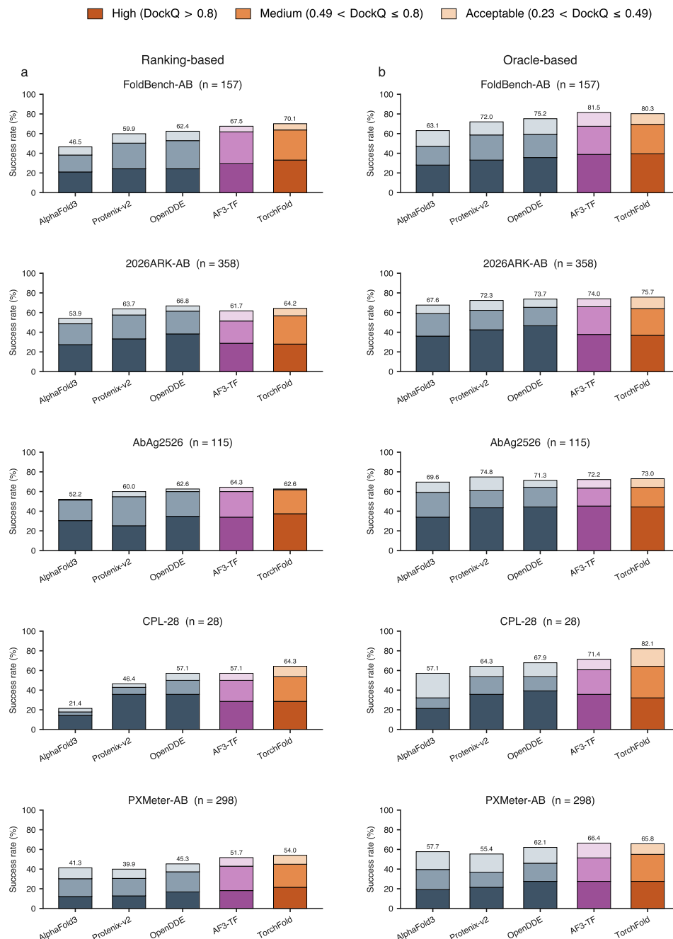
Figure 4 Antibody-antigen DockQ success. (a) Ranking-based and (b) oracle-based success on FoldBench-AB, 2026ARK-AB, AbAg2526, CPL-28 and PXMeter-AB. n is the number of scored interfaces. Stacked segments: high (DockQ > 0.8), medium (0.49 < DockQ ≤ 0.8), acceptable (0.23 < DockQ ≤ 0.49).
