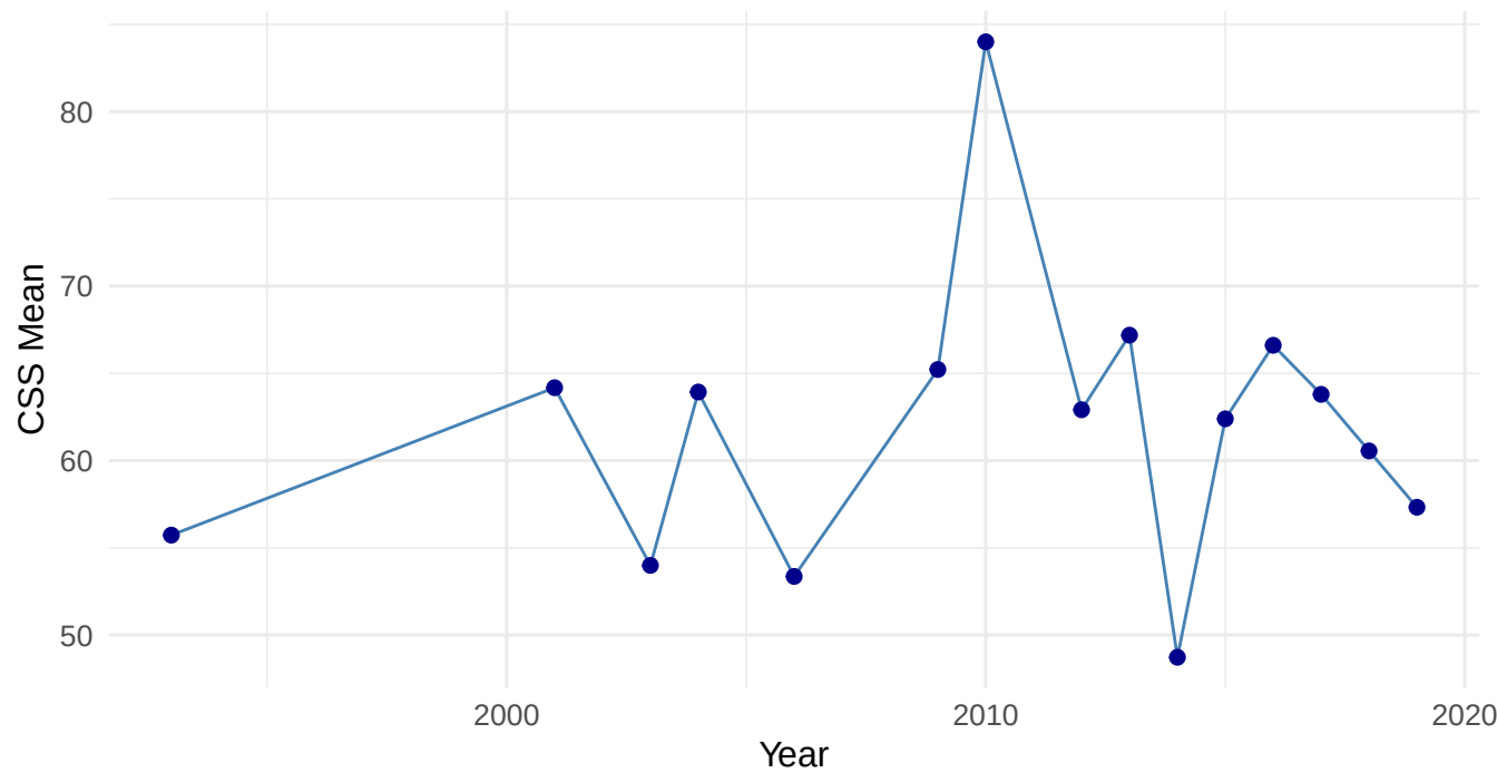
Benin: CSS Mean over time
