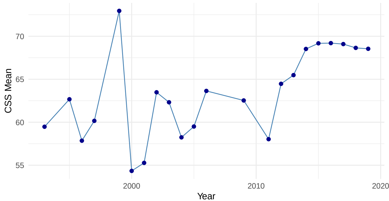
Costa Rica: CSS Mean over time
