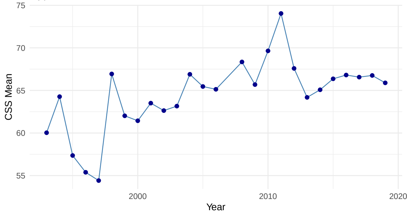
Cyprus: CSS Mean over time
