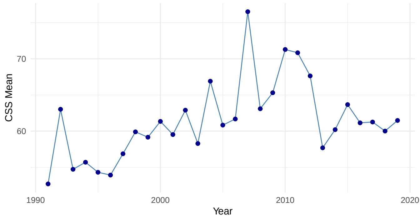
Egypt: CSS Mean over time
