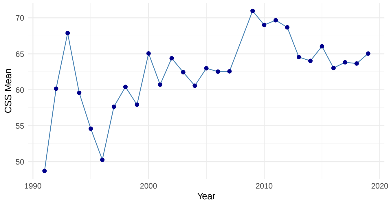
Lebanon: CSS Mean over time
