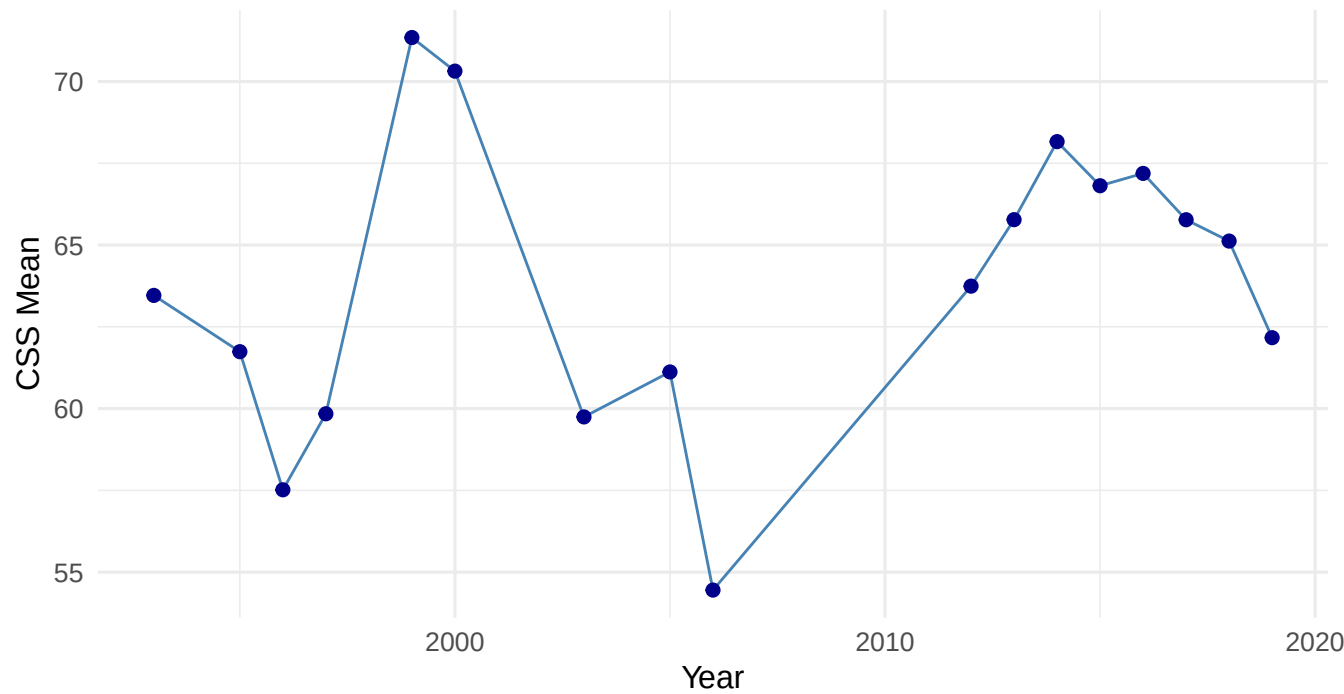
Nicaragua: CSS Mean over time
