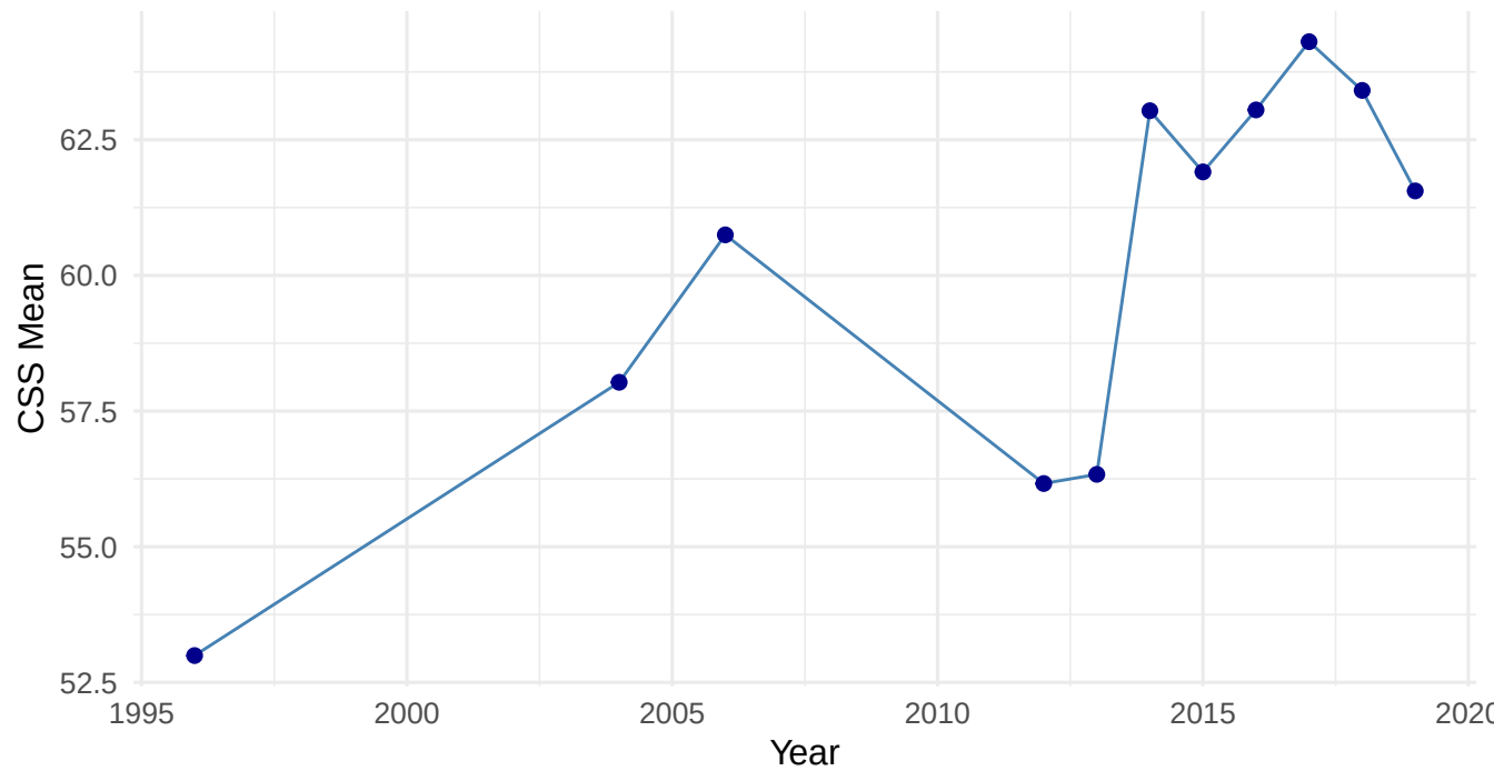
Rwanda: CSS Mean over time
