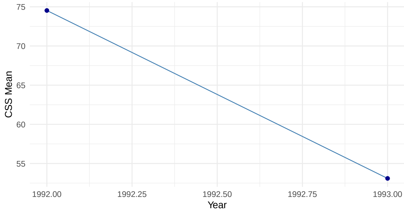
Senegambia: CSS Mean over time
