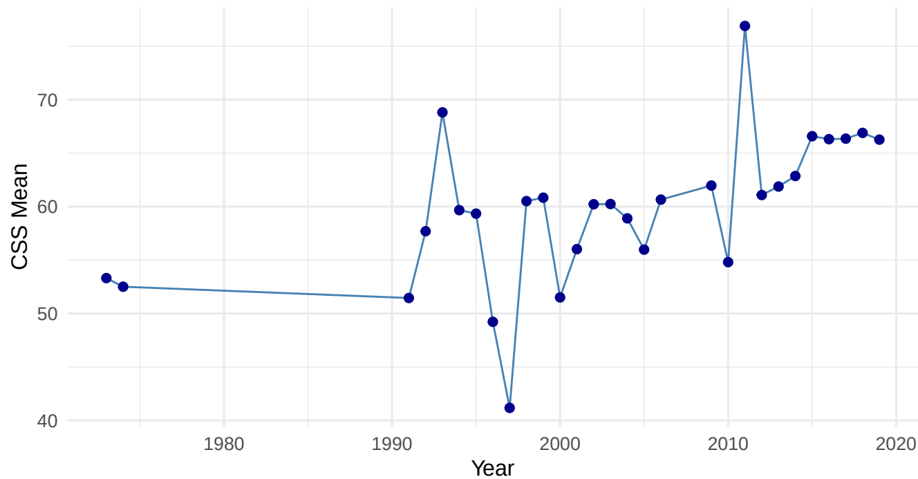
Serbia: CSS Mean over time
