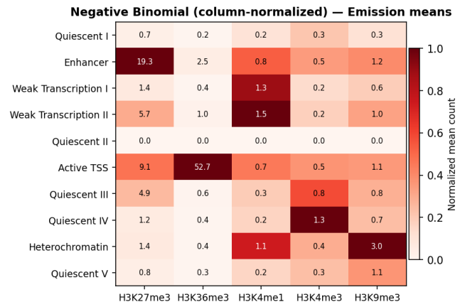
Figure 1 Emission parameter heatmaps for the NB model. Rows are inferred chromatin states labeled with their biological identity; columns are histone marks. Values are column-normalized mean counts. Equivalent figures for Bernoulli and Poisson are provided as supplementary material.
