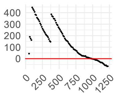
(b) p=50, n=50
