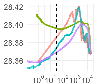
(h) p=200, n=200
