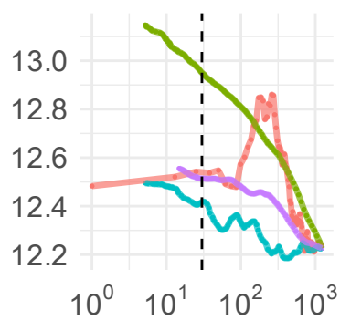
(a) p=50, n=25
