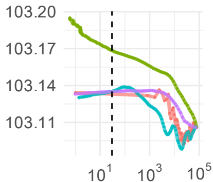
(j) p=400, n=200
