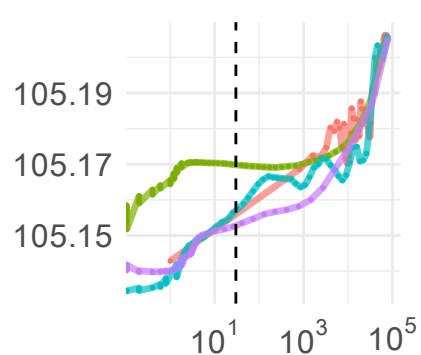
(k) p=400, n=400
