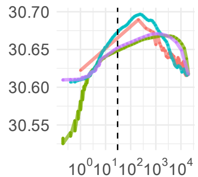
(i) p=200, n=400
