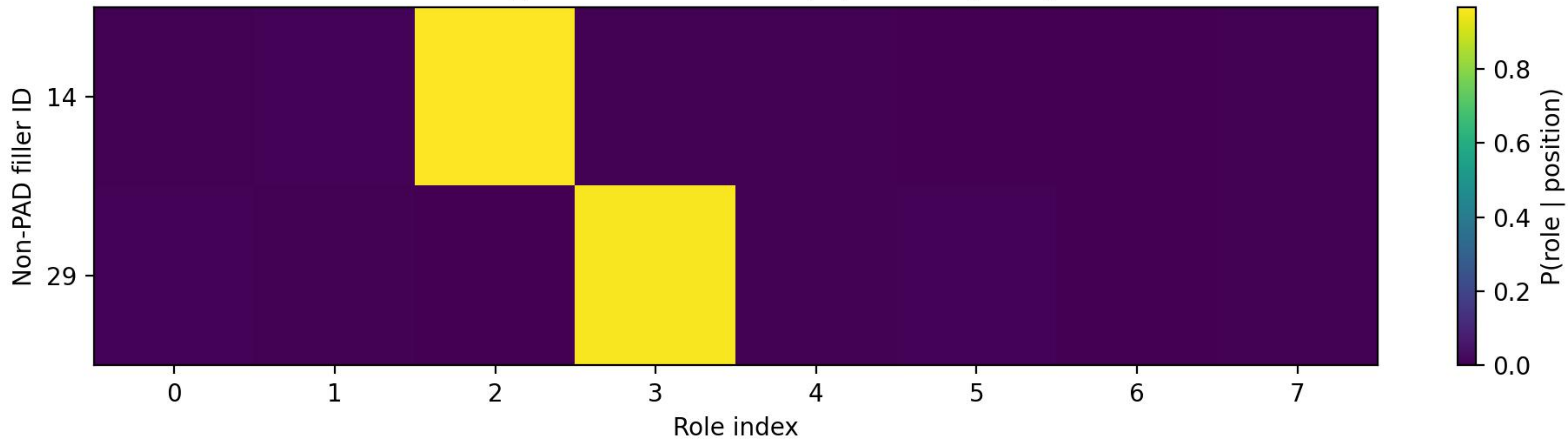
ROLE assignment distribution | epoch 50 | image 9
