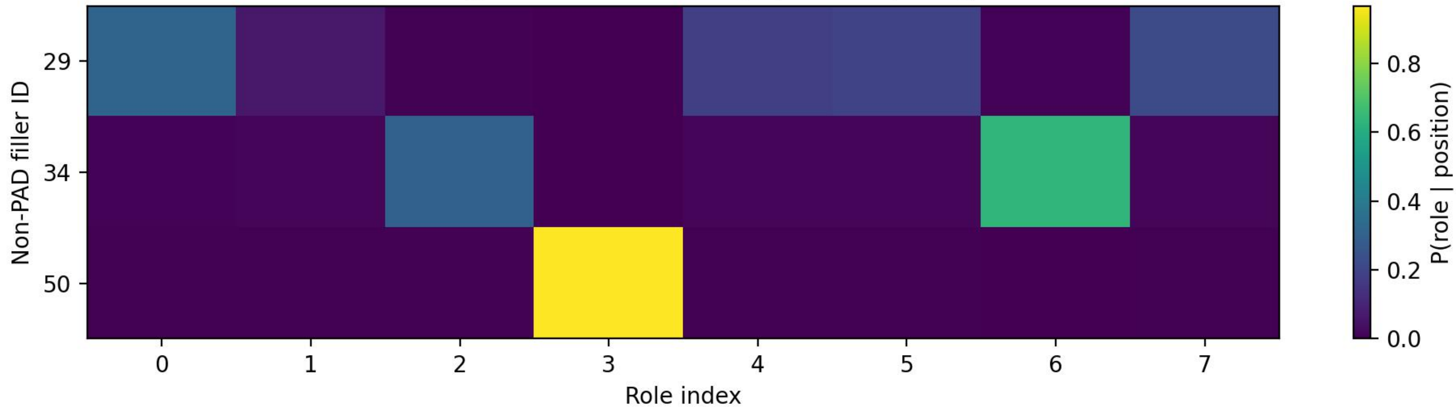
ROLE assignment distribution | epoch 50 | image 11
