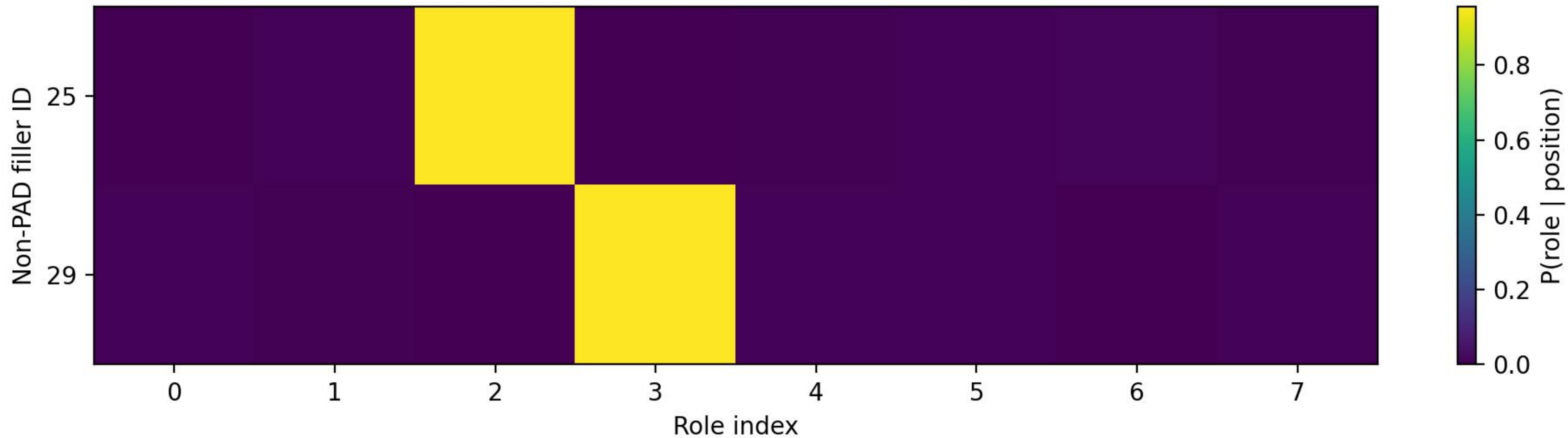
ROLE assignment distribution | epoch 50 | image 10
