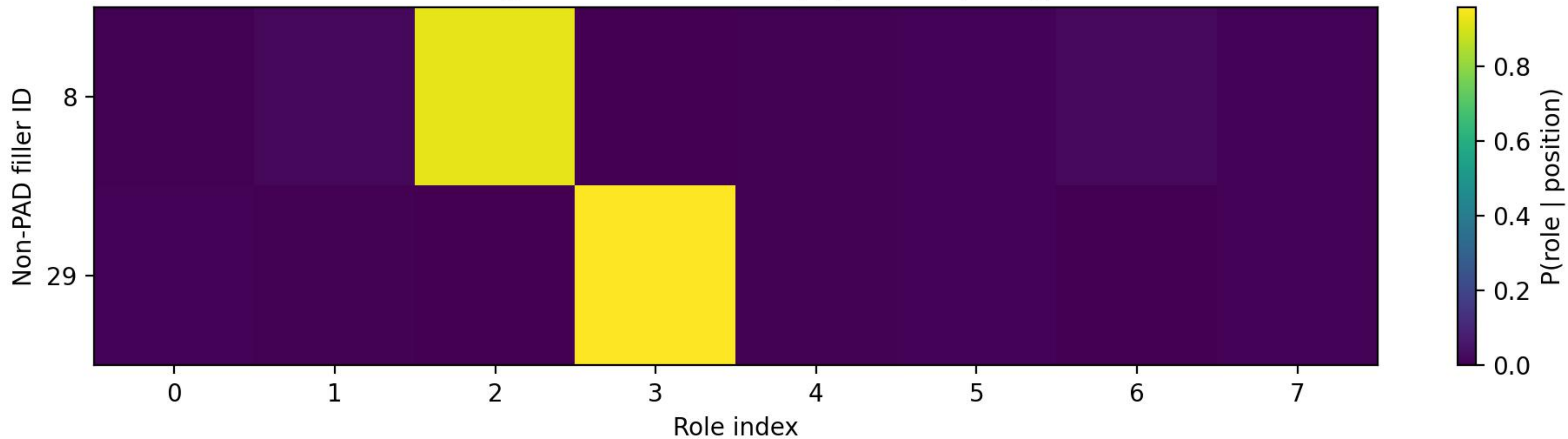
ROLE assignment distribution | epoch 50 | image 19
