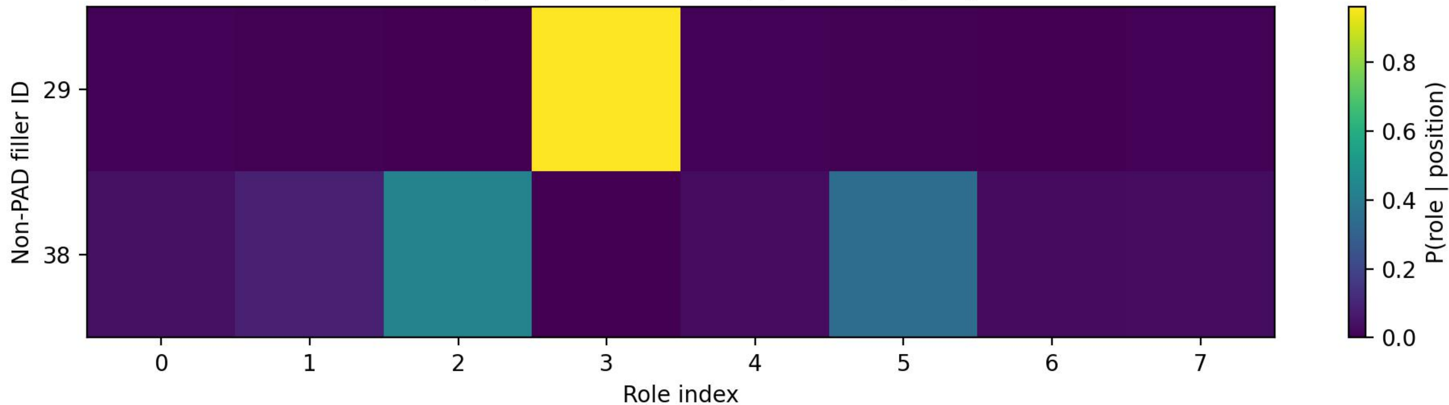
ROLE assignment distribution | epoch 50 | image 8
