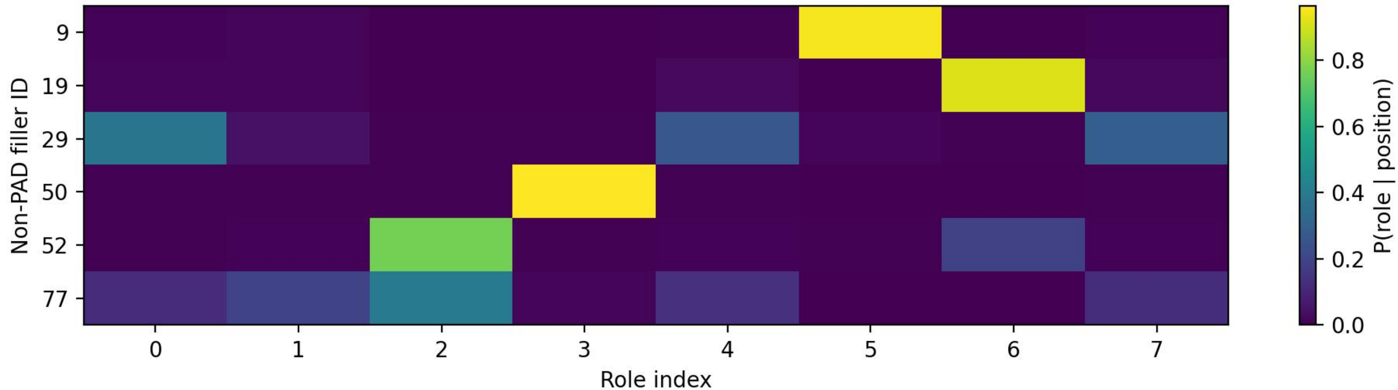
ROLE assignment distribution | epoch 50 | image 16
