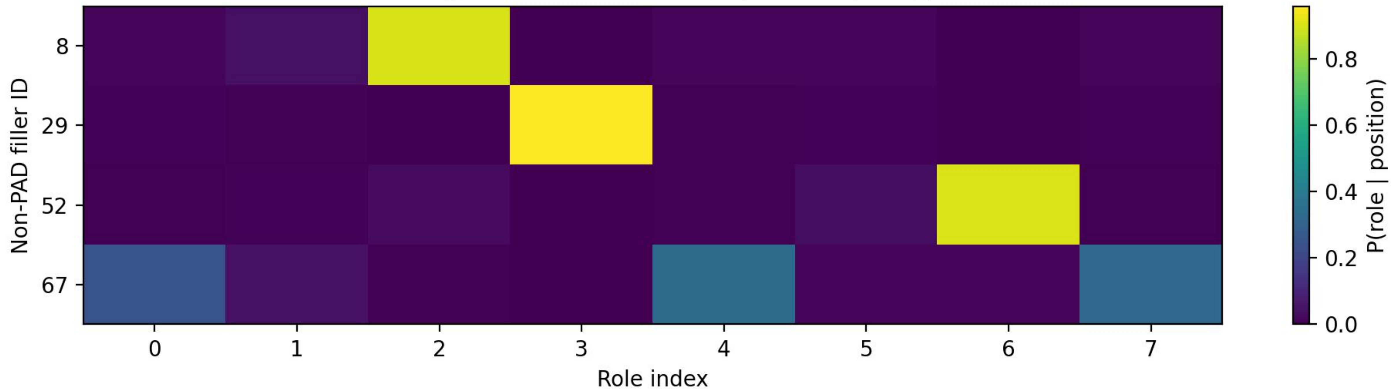
ROLE assignment distribution | epoch 50 | image 12
