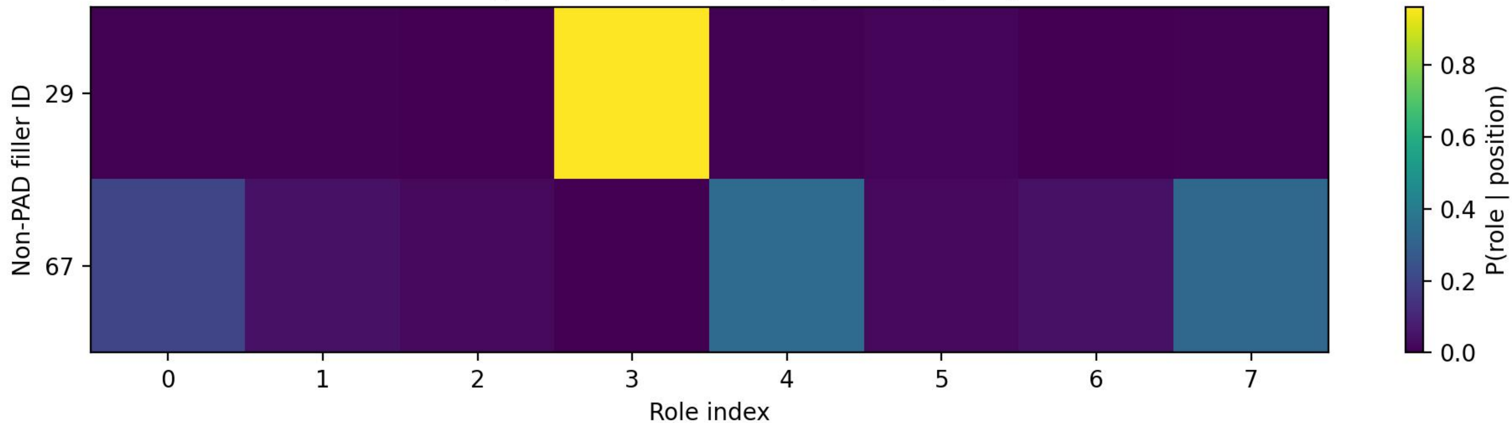
ROLE assignment distribution | epoch 50 | image 2
