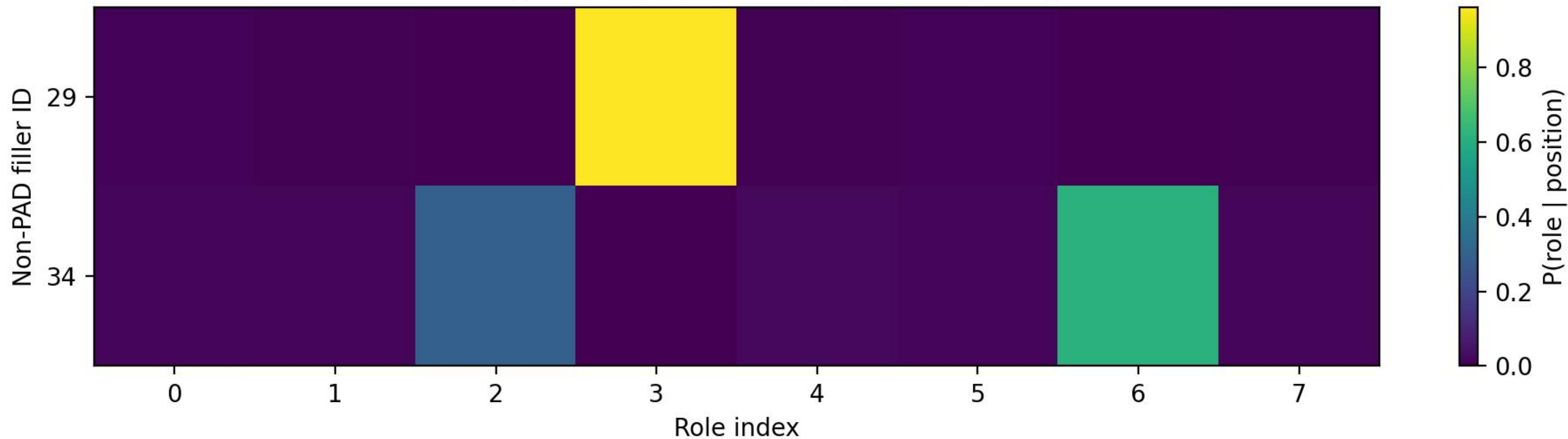
ROLE assignment distribution | epoch 50 | image 3
