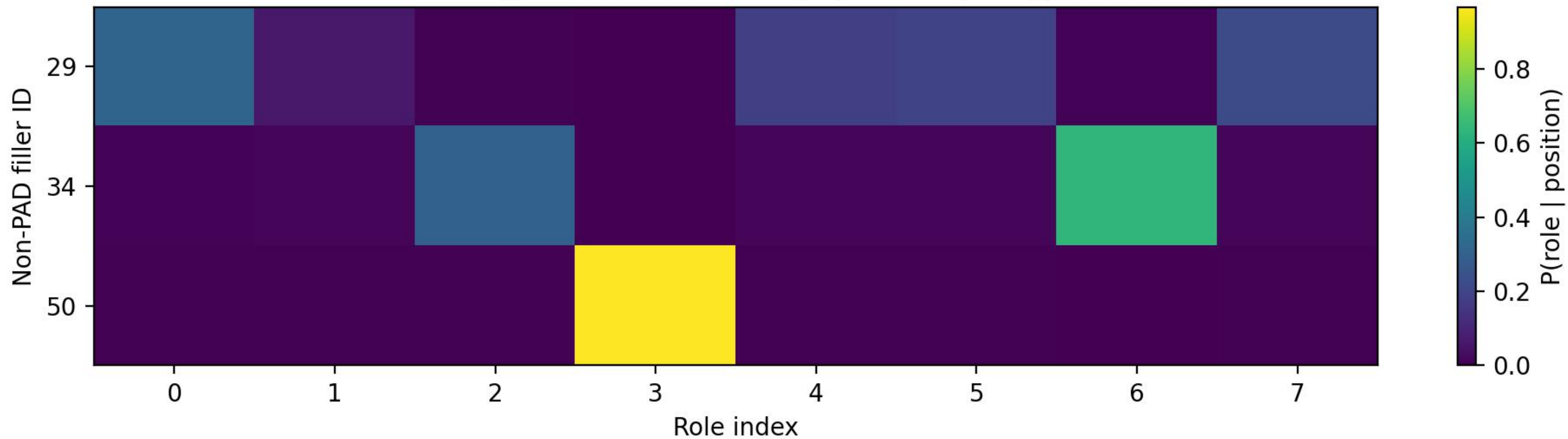
ROLE assignment distribution | epoch 50 | image 20
