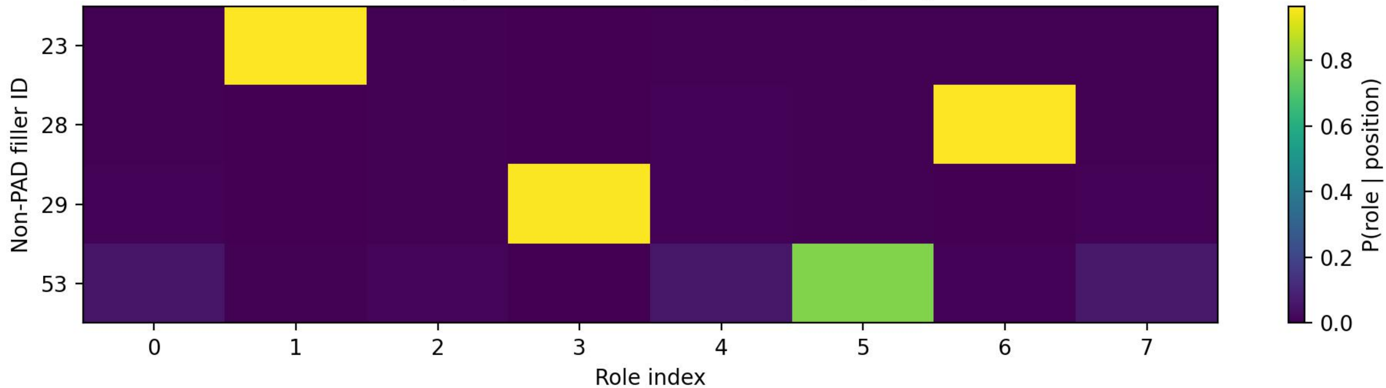
ROLE assignment distribution | epoch 50 | image 5
