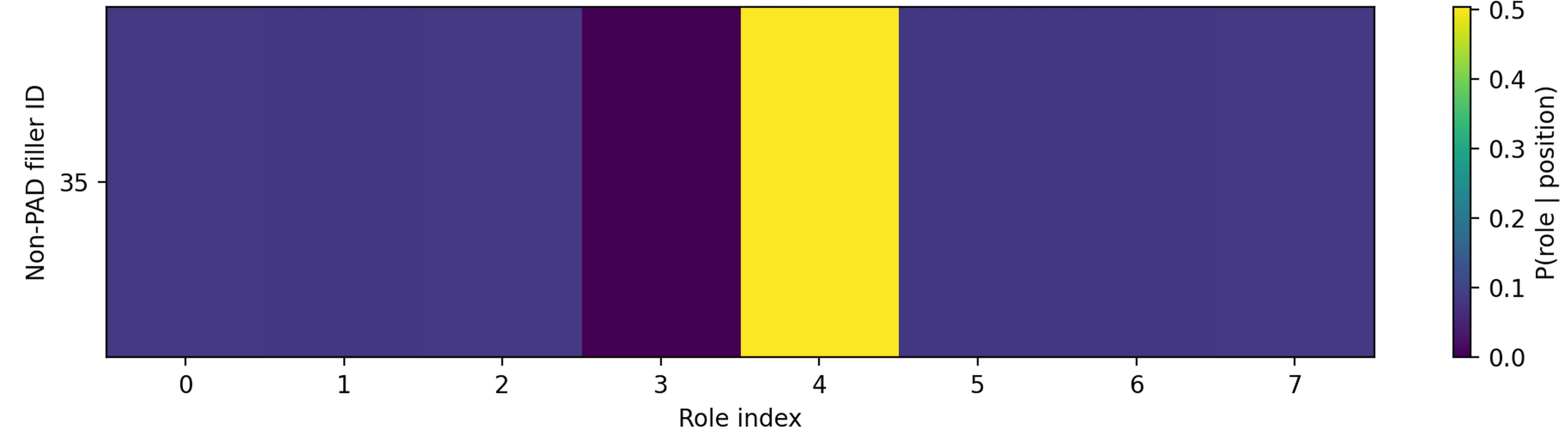
ROLE assignment distribution | epoch 150 | image 42844
