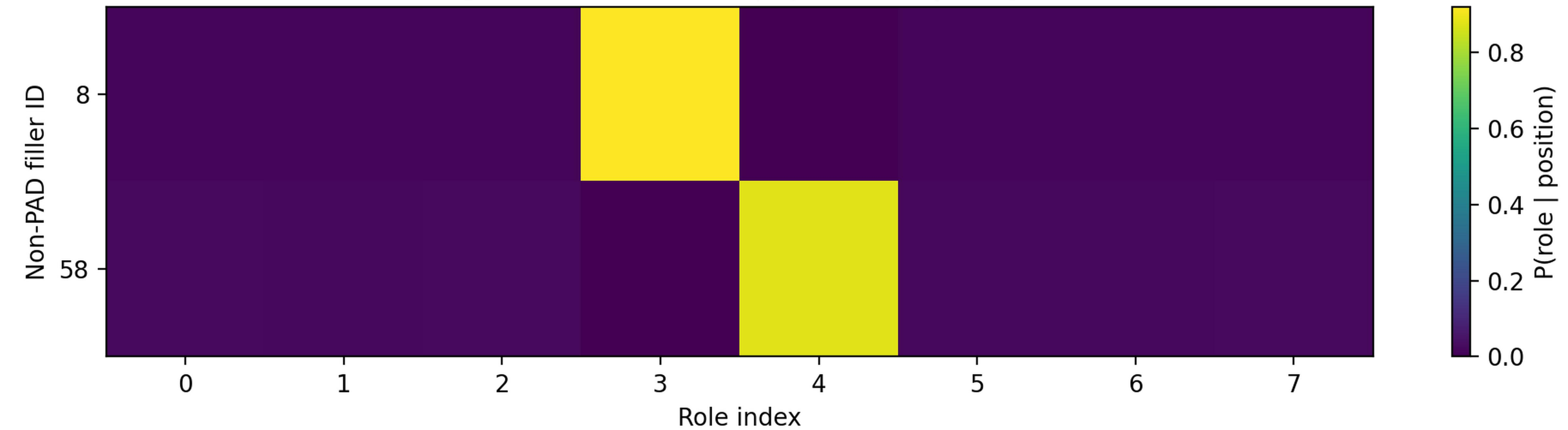
ROLE assignment distribution | epoch 150 | image 378911
