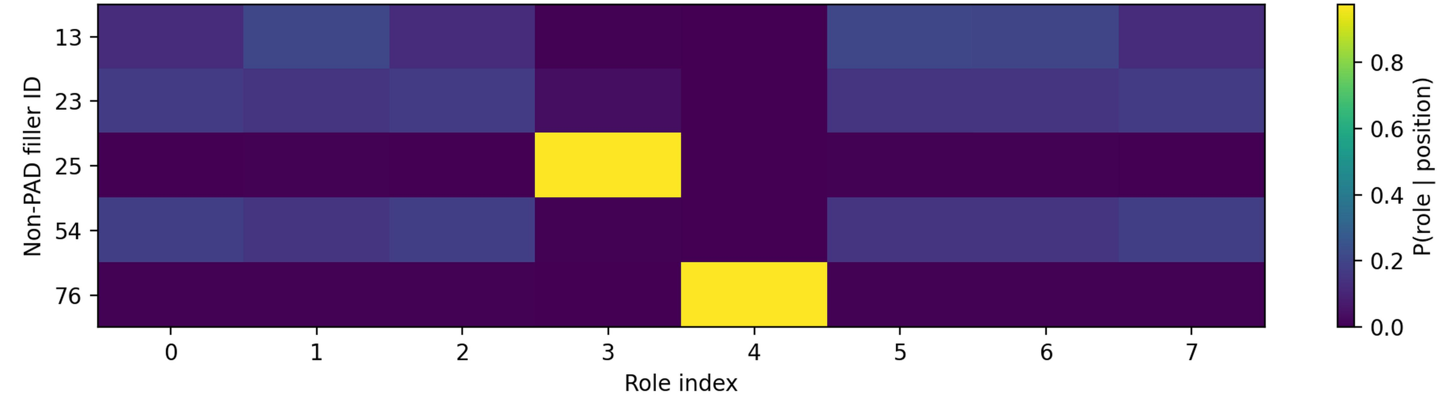
ROLE assignment distribution | epoch 150 | image 324611
