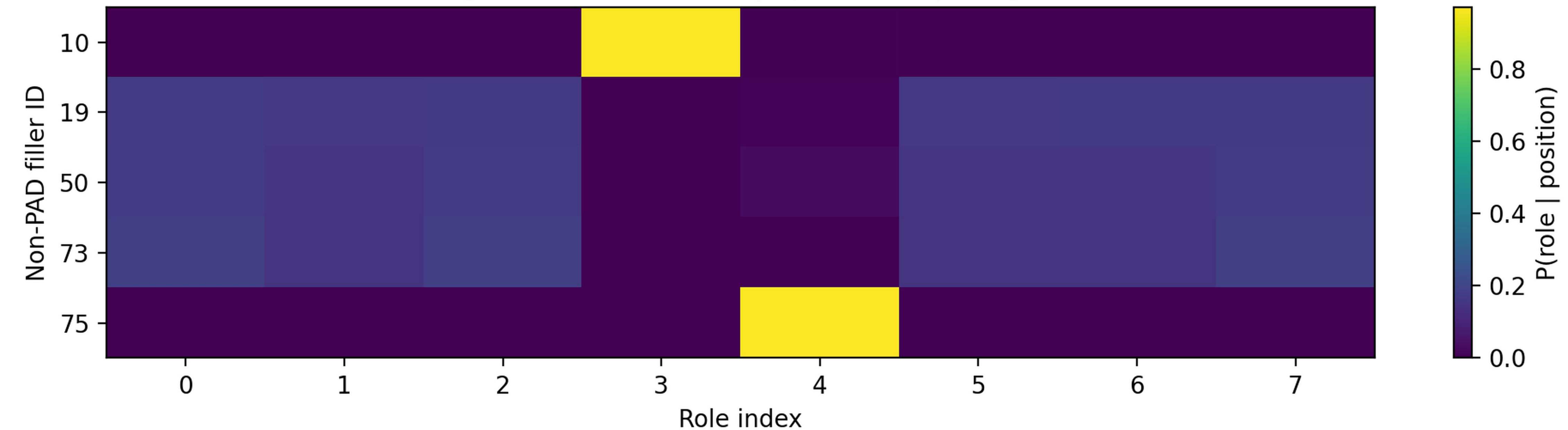
ROLE assignment distribution | epoch 150 | image 301926
