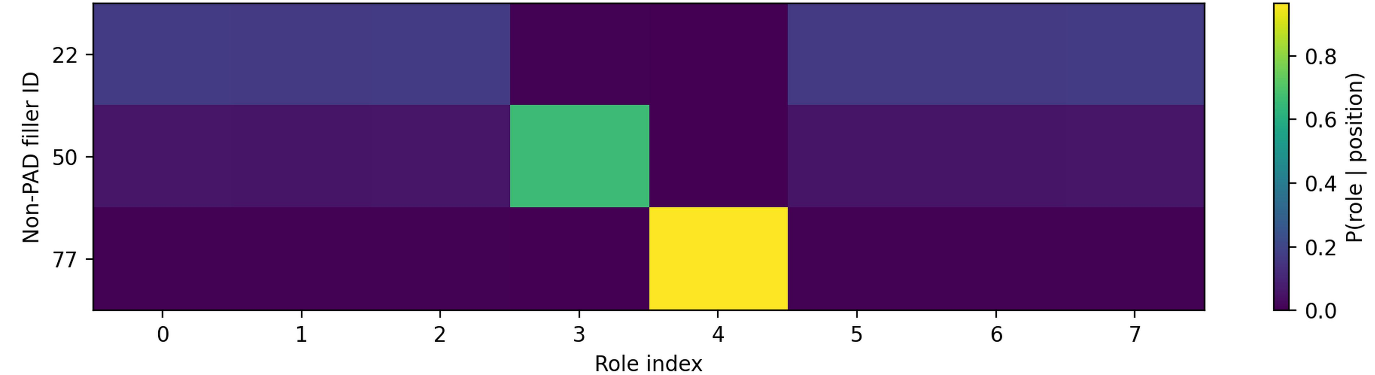
ROLE assignment distribution | epoch 150 | image 358923
