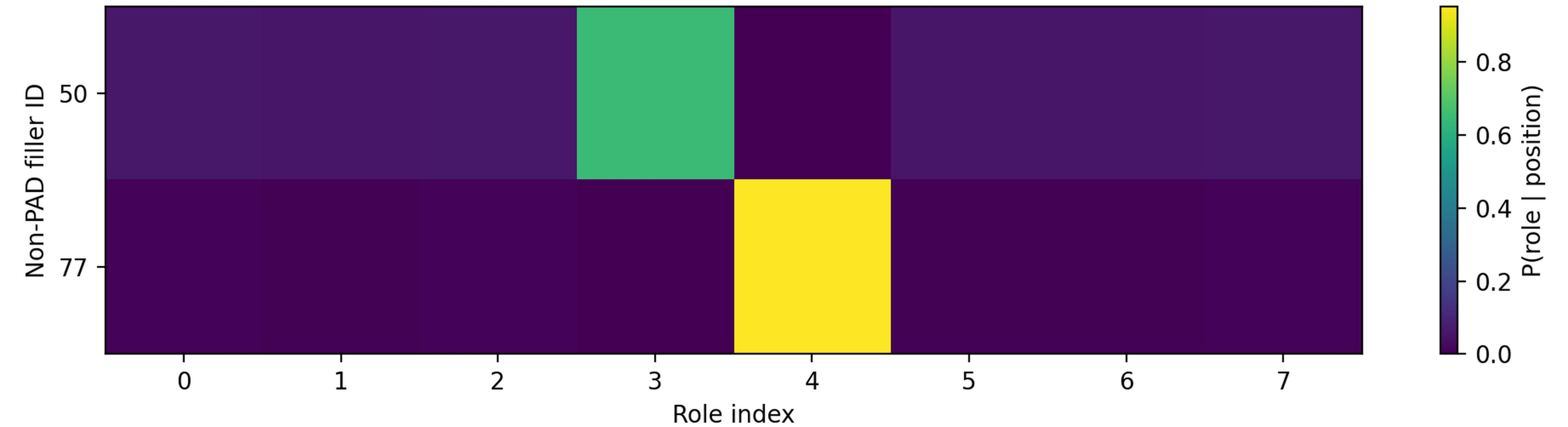
ROLE assignment distribution | epoch 150 | image 461983
