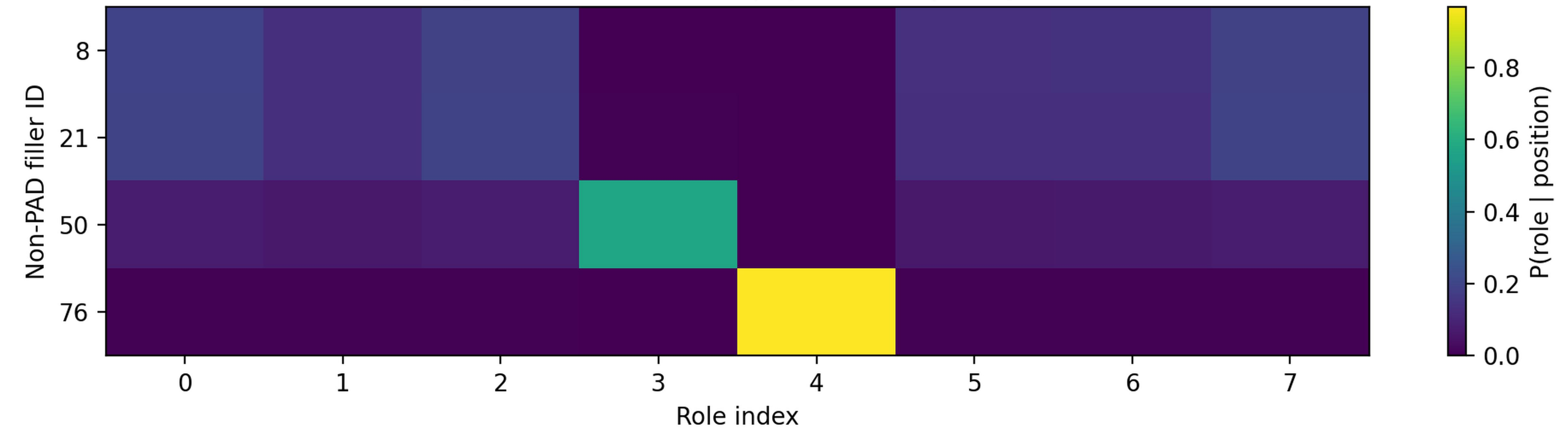
ROLE assignment distribution | epoch 150 | image 452498
