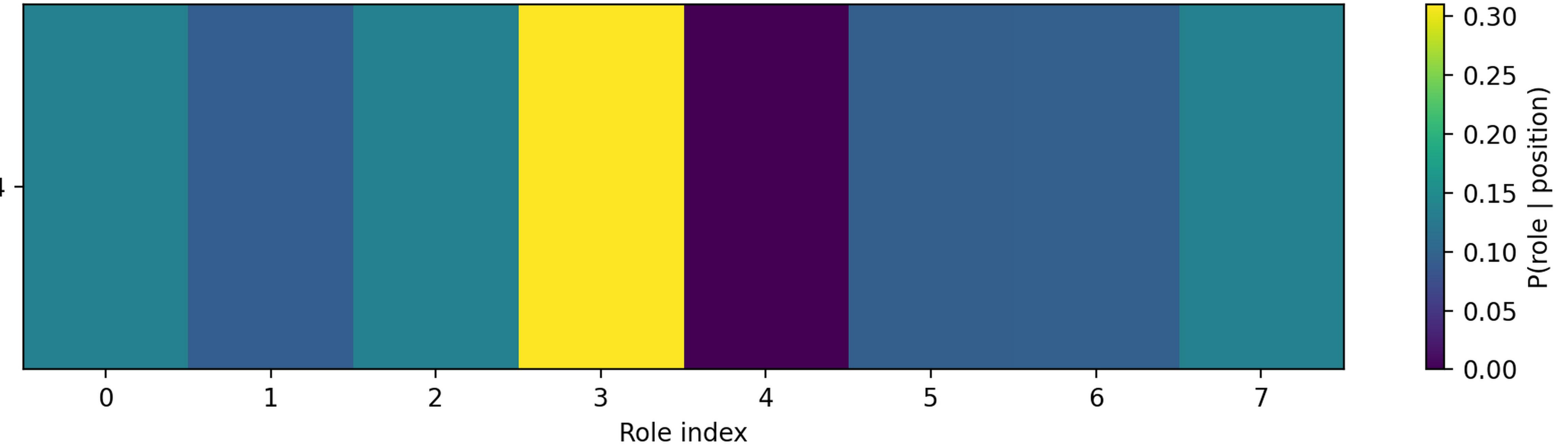
ROLE assignment distribution | epoch 150 | image 16898
