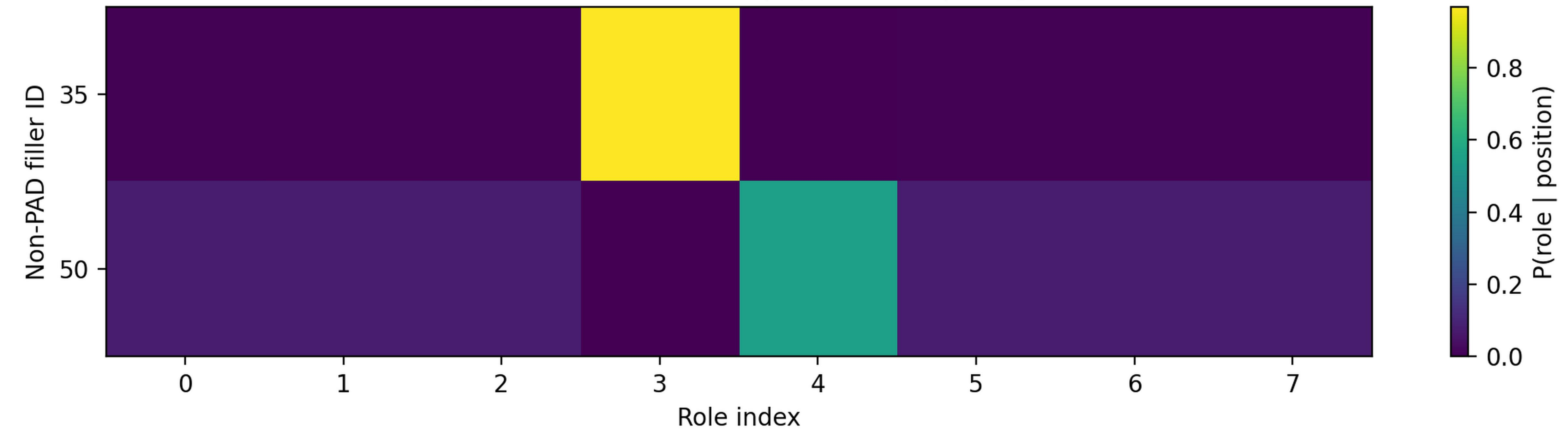
ROLE assignment distribution | epoch 150 | image 99313
