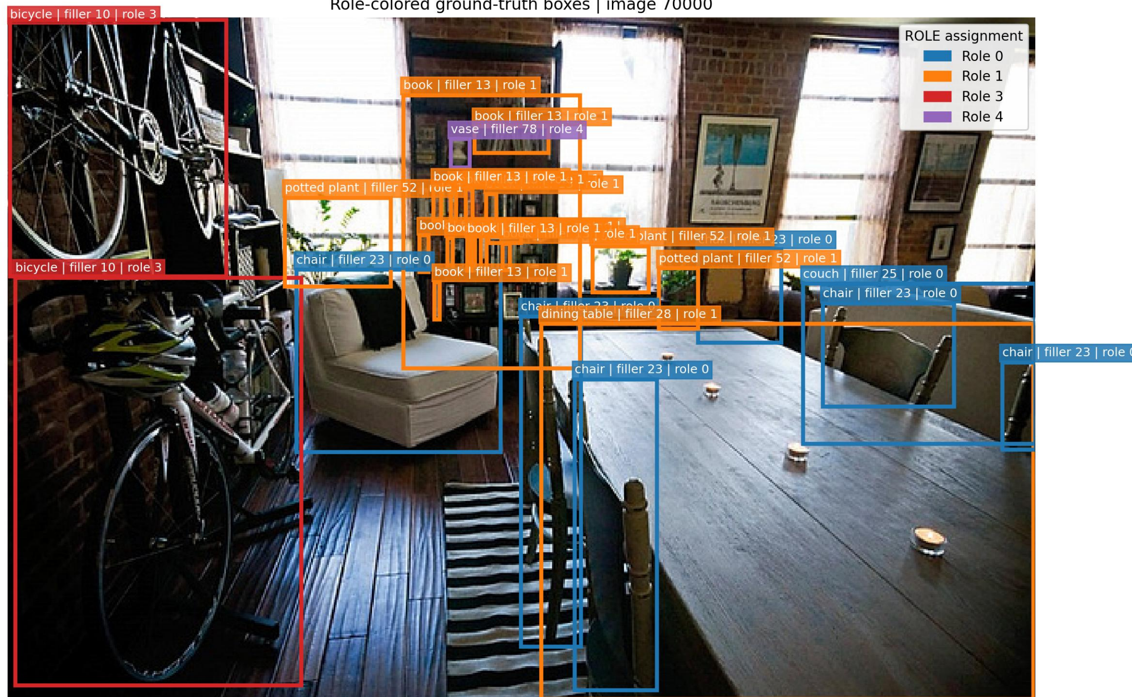
Role-colored ground-truth boxes | image 70000
