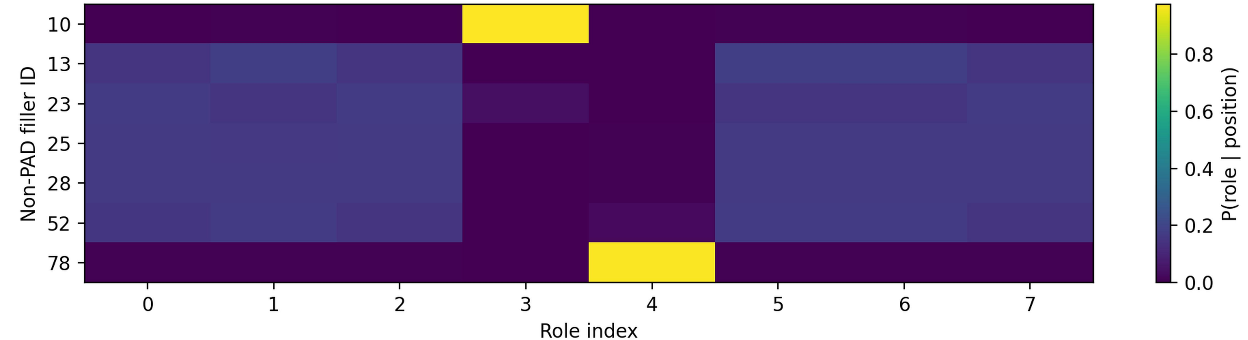
ROLE assignment distribution | epoch 150 | image 70000
