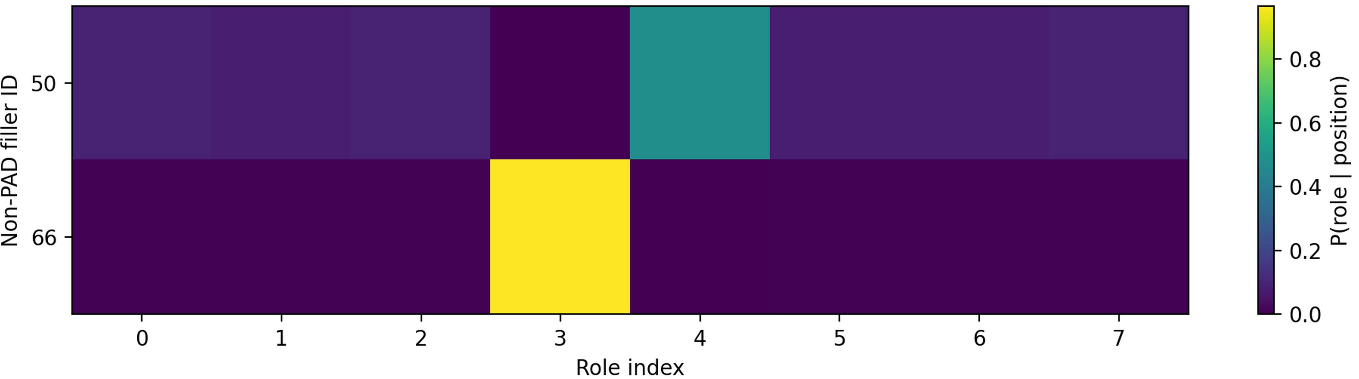
ROLE assignment distribution | epoch 150 | image 340658
