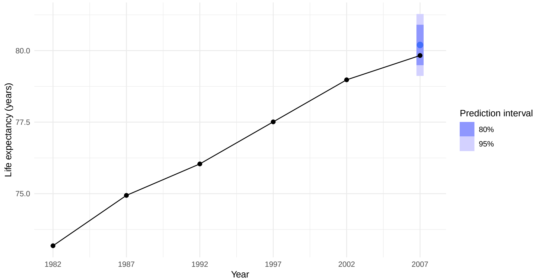
Austria: random walk with drift forecast for 2007 vs actual
