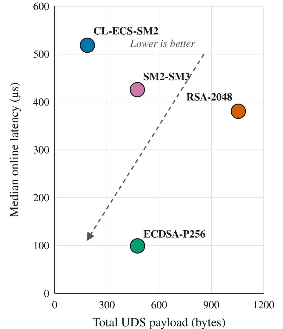
(c) Latency–payload trade-off
