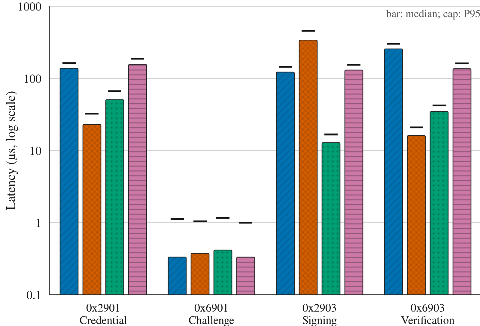
(a) Online latency by protocol phase
